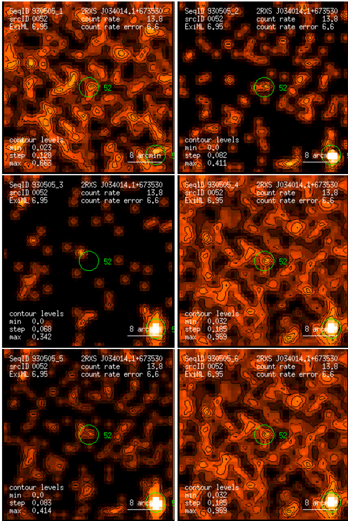
Figure 52: RASS 930505: detection 0052: band rate images, Gaussian filter: (1) PSPC channels 11 – 41, (2) 52 – 90, (3) 91 – 201, (4) 11 – 235, (5) 52 – 201, (6) 11 – 201. Broad band rates in counts/ks. Band rate contour levels in counts/ks/arcmin 2 .
