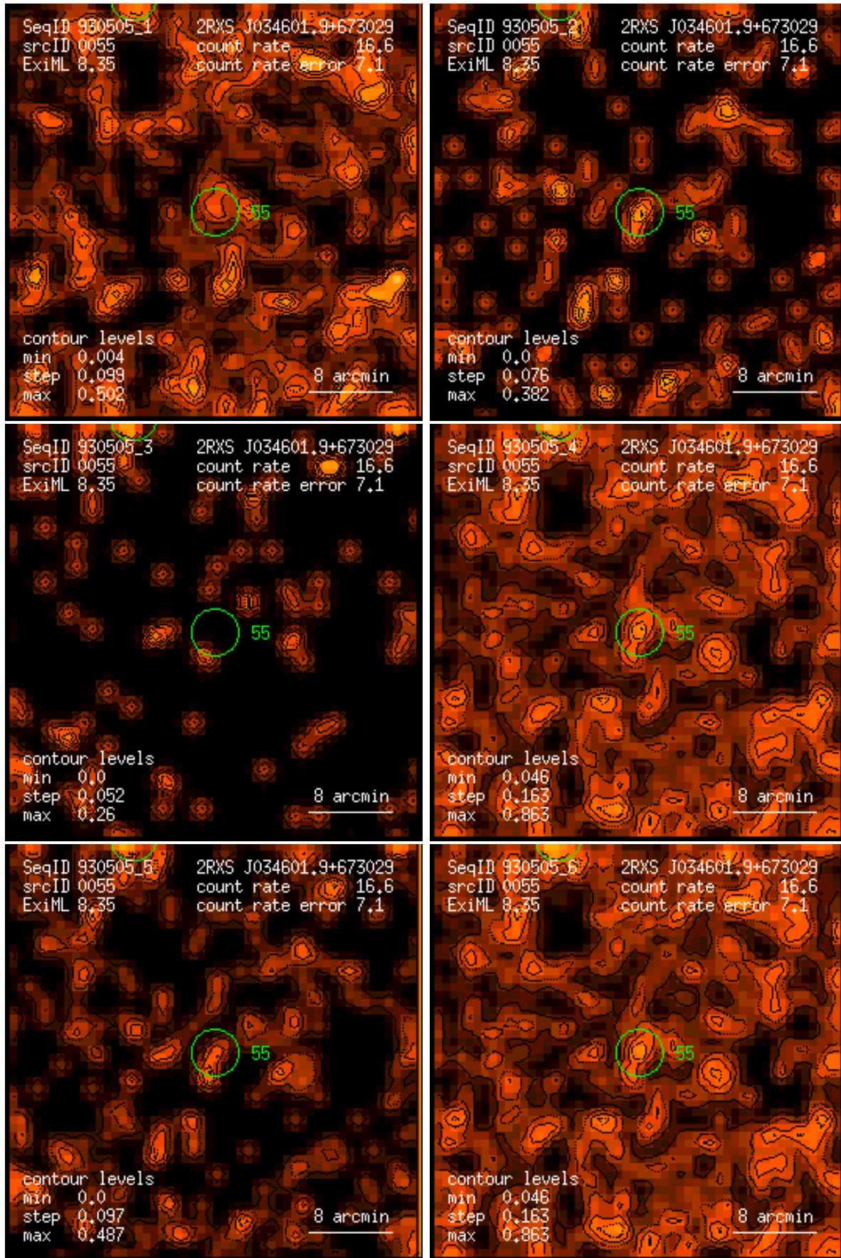
Figure 55: RASS 930505: detection 0055: band rate images, Gaussian filter: (1) PSPC channels 11 – 41, (2) 52 – 90, (3) 91 – 201, (4) 11 – 235, (5) 52 – 201, (6) 11 – 201. Broad band rates in counts/ks. Band rate contour levels in counts/ks/arcmin 2 .
