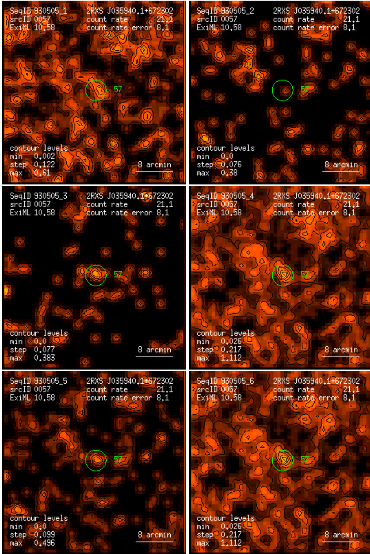
Figure 57: RASS 930505: detection 0057: band rate images, Gaussian filter: (1) PSPC channels 11 – 41, (2) 52 – 90, (3) 91 – 201, (4) 11 – 235, (5) 52 – 201, (6) 11 – 201. Broad band rates in counts/ks. Band rate contour levels in counts/ks/arcmin 2 .
