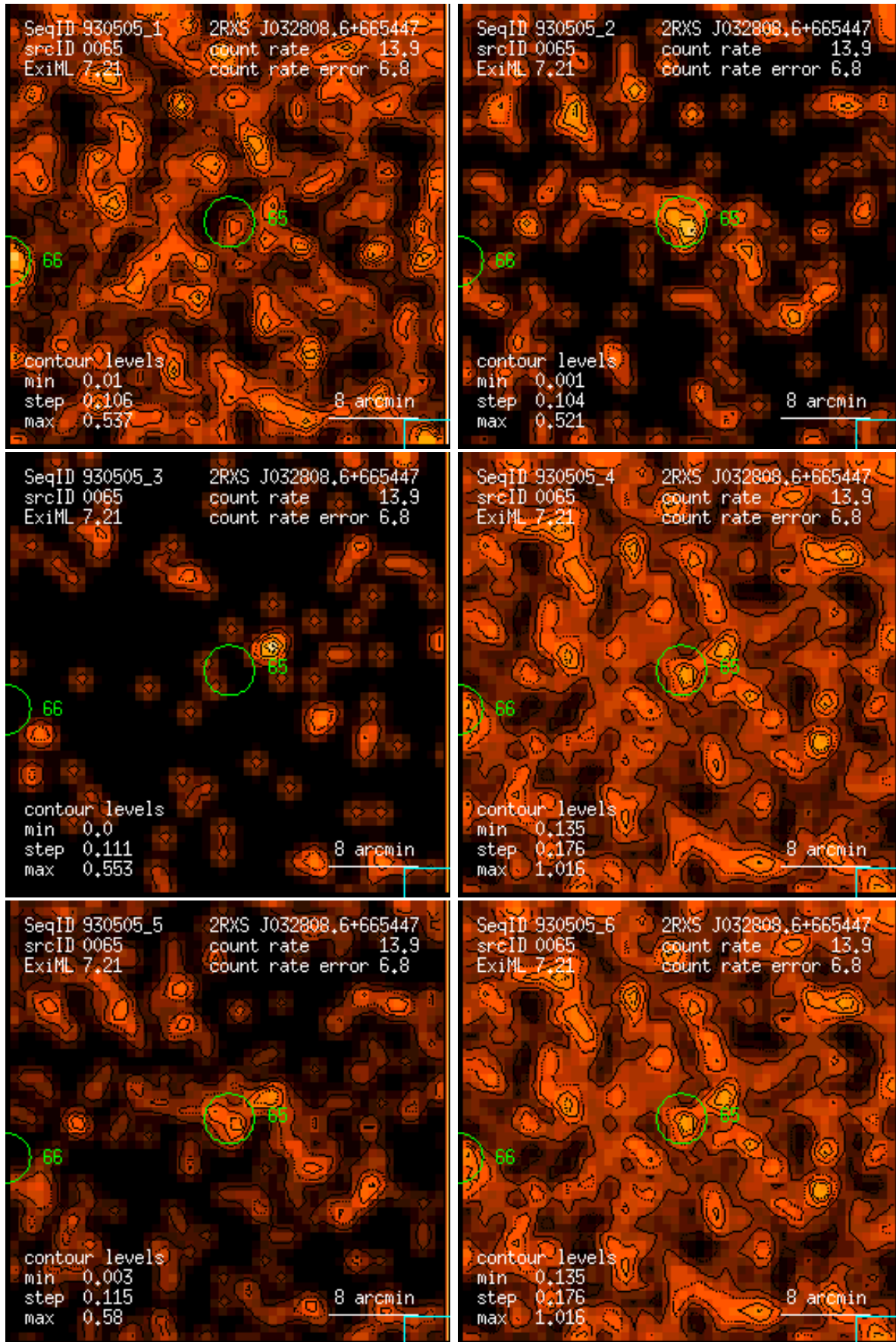
Figure 65: RASS 930505: detection 0065: band rate images, Gaussian filter: (1) PSPC channels 11 – 41, (2) 52 – 90, (3) 91 – 201, (4) 11 – 235, (5) 52 – 201, (6) 11 – 201. Broad band rates in counts/ks. Band rate contour levels in counts/ks/arcmin 2 .
