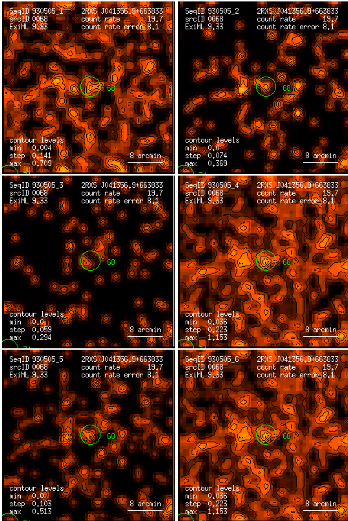
Figure 68: RASS 930505: detection 0068: band rate images, Gaussian filter: (1) PSPC channels 11 – 41, (2) 52 – 90, (3) 91 – 201, (4) 11 – 235, (5) 52 – 201, (6) 11 – 201. Broad band rates in counts/ks. Band rate contour levels in counts/ks/arcmin 2 .
