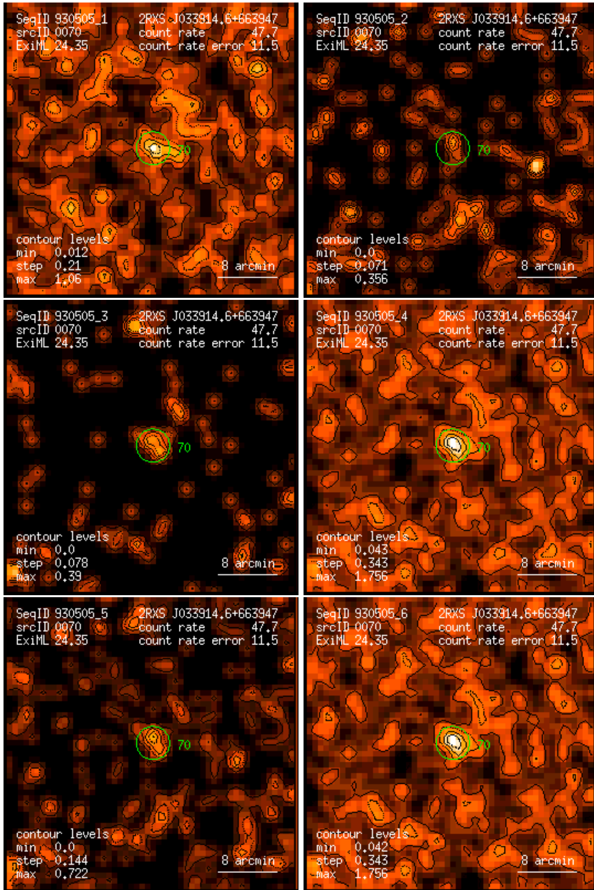
Figure 70: RASS 930505: detection 0070: band rate images, Gaussian filter: (1) PSPC channels 11 – 41, (2) 52 – 90, (3) 91 – 201, (4) 11 – 235, (5) 52 – 201, (6) 11 – 201. Broad band rates in counts/ks. Band rate contour levels in counts/ks/arcmin 2 .
