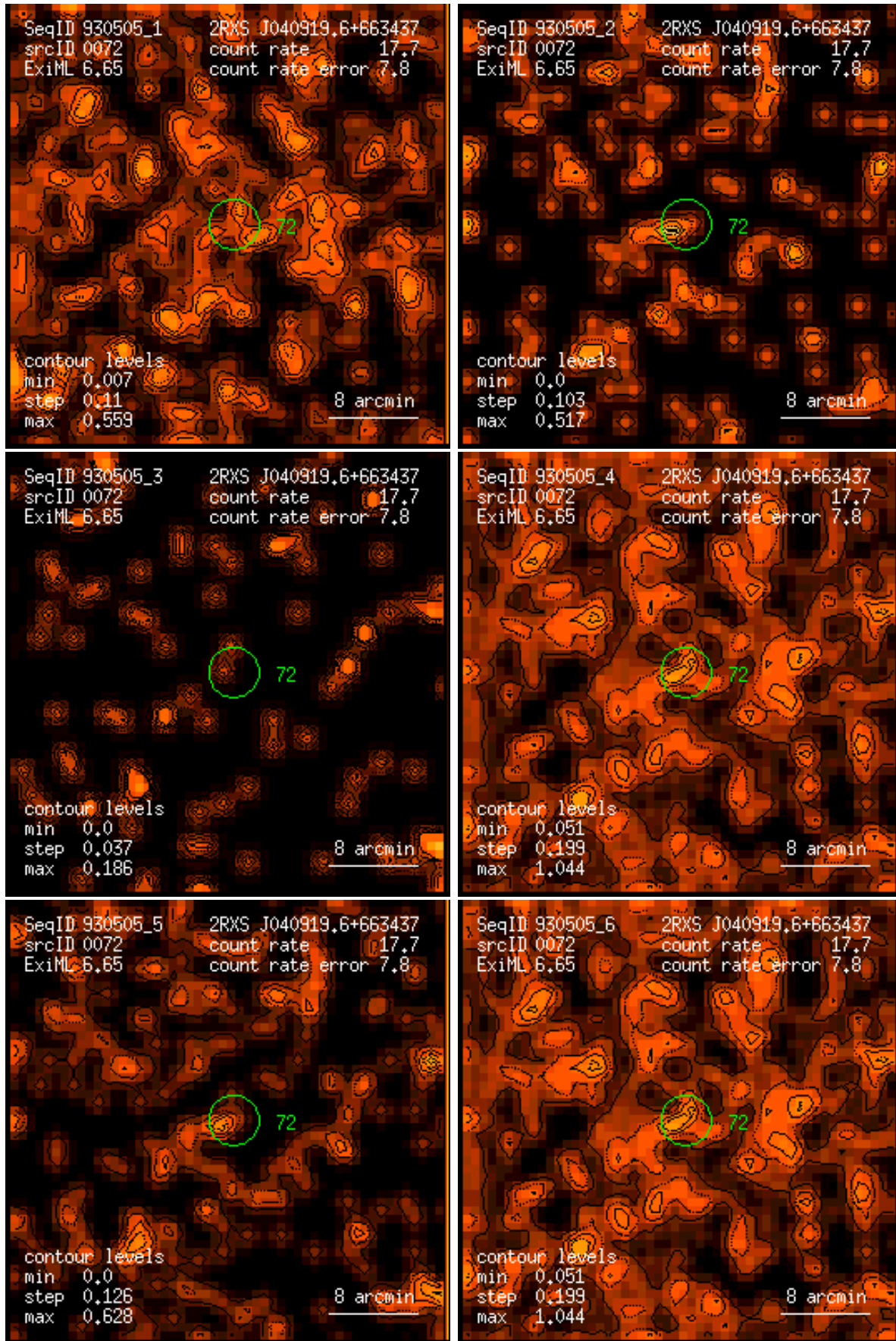
Figure 72: RASS 930505: detection 0072: band rate images, Gaussian filter: (1) PSPC channels 11 – 41, (2) 52 – 90, (3) 91 – 201, (4) 11 – 235, (5) 52 – 201, (6) 11 – 201. Broad band rates in counts/ks. Band rate contour levels in counts/ks/arcmin 2 .
