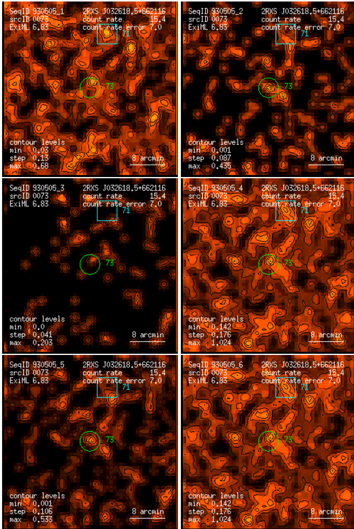
Figure 73: RASS 930505: detection 0073: band rate images, Gaussian filter: (1) PSPC channels 11 – 41, (2) 52 – 90, (3) 91 – 201, (4) 11 – 235, (5) 52 – 201, (6) 11 – 201. Broad band rates in counts/ks. Band rate contour levels in counts/ks/arcmin 2 .
