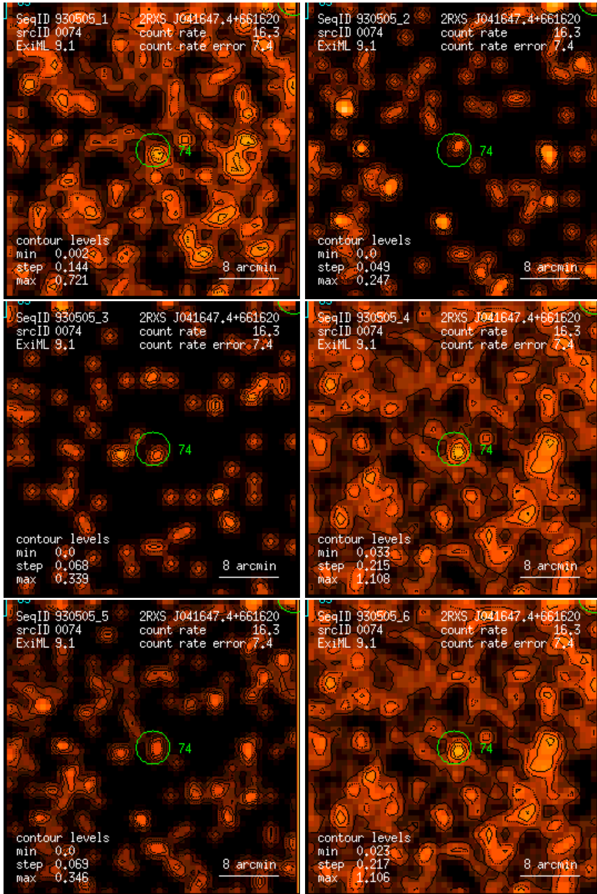
Figure 74: RASS 930505: detection 0074: band rate images, Gaussian filter: (1) PSPC channels 11 – 41, (2) 52 – 90, (3) 91 – 201, (4) 11 – 235, (5) 52 – 201, (6) 11 – 201. Broad band rates in counts/ks. Band rate contour levels in counts/ks/arcmin 2 .
