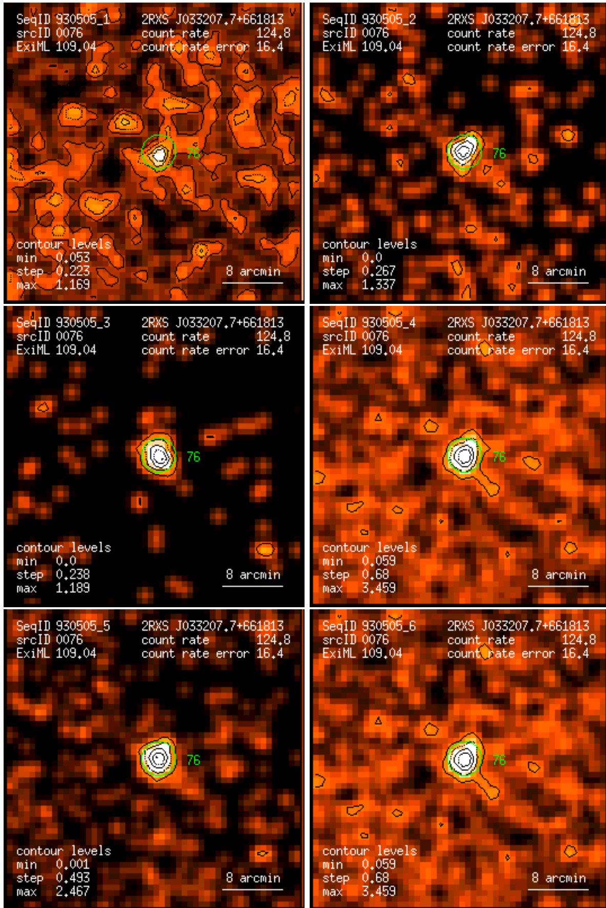
Figure 76: RASS 930505: detection 0076: band rate images, Gaussian filter: (1) PSPC channels 11 – 41, (2) 52 – 90, (3) 91 – 201, (4) 11 – 235, (5) 52 – 201, (6) 11 – 201. Broad band rates in counts/ks. Band rate contour levels in counts/ks/arcmin 2 .
