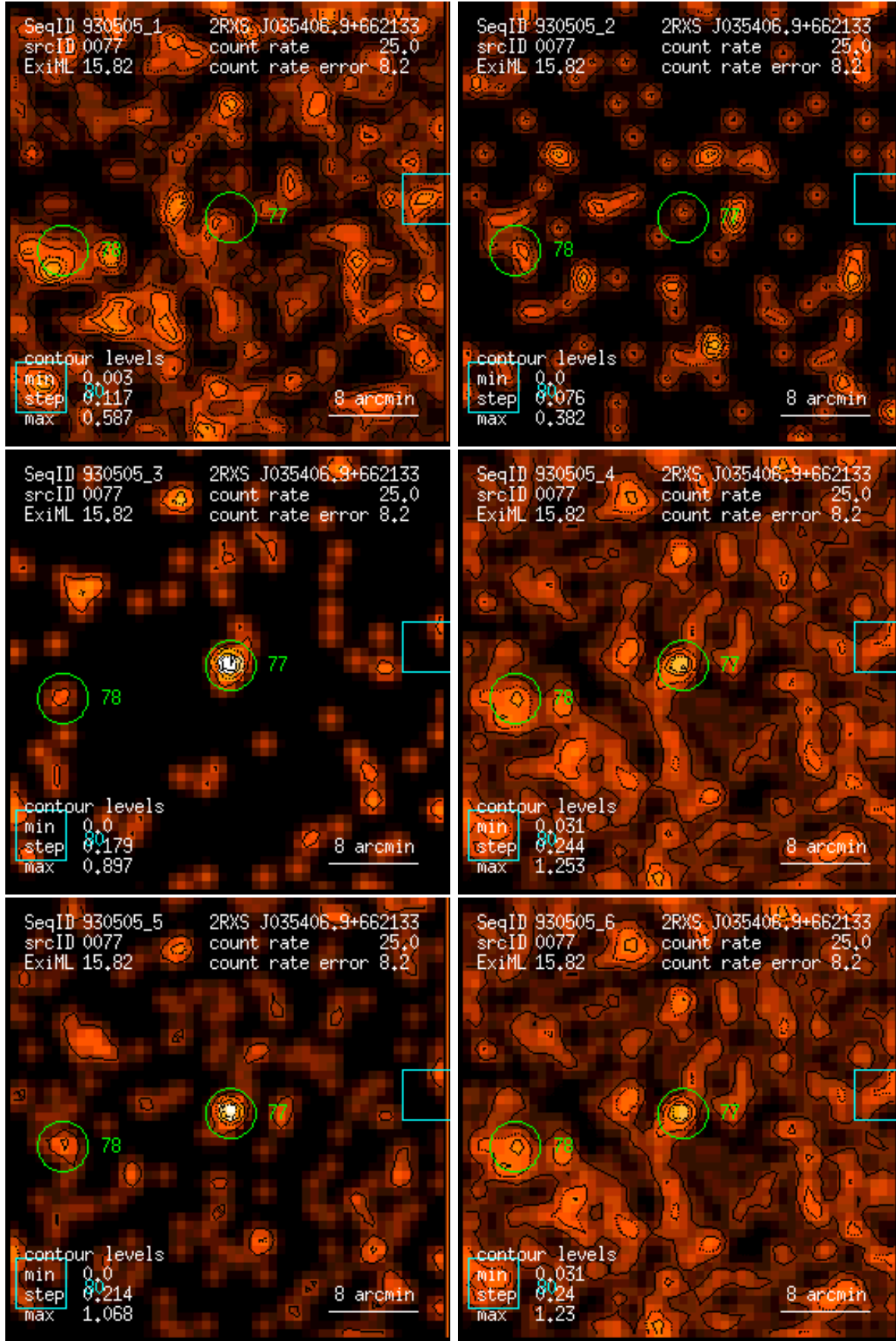
Figure 77: RASS 930505: detection 0077: band rate images, Gaussian filter: (1) PSPC channels 11 – 41, (2) 52 – 90, (3) 91 – 201, (4) 11 – 235, (5) 52 – 201, (6) 11 – 201. Broad band rates in counts/ks. Band rate contour levels in counts/ks/arcmin 2 .
