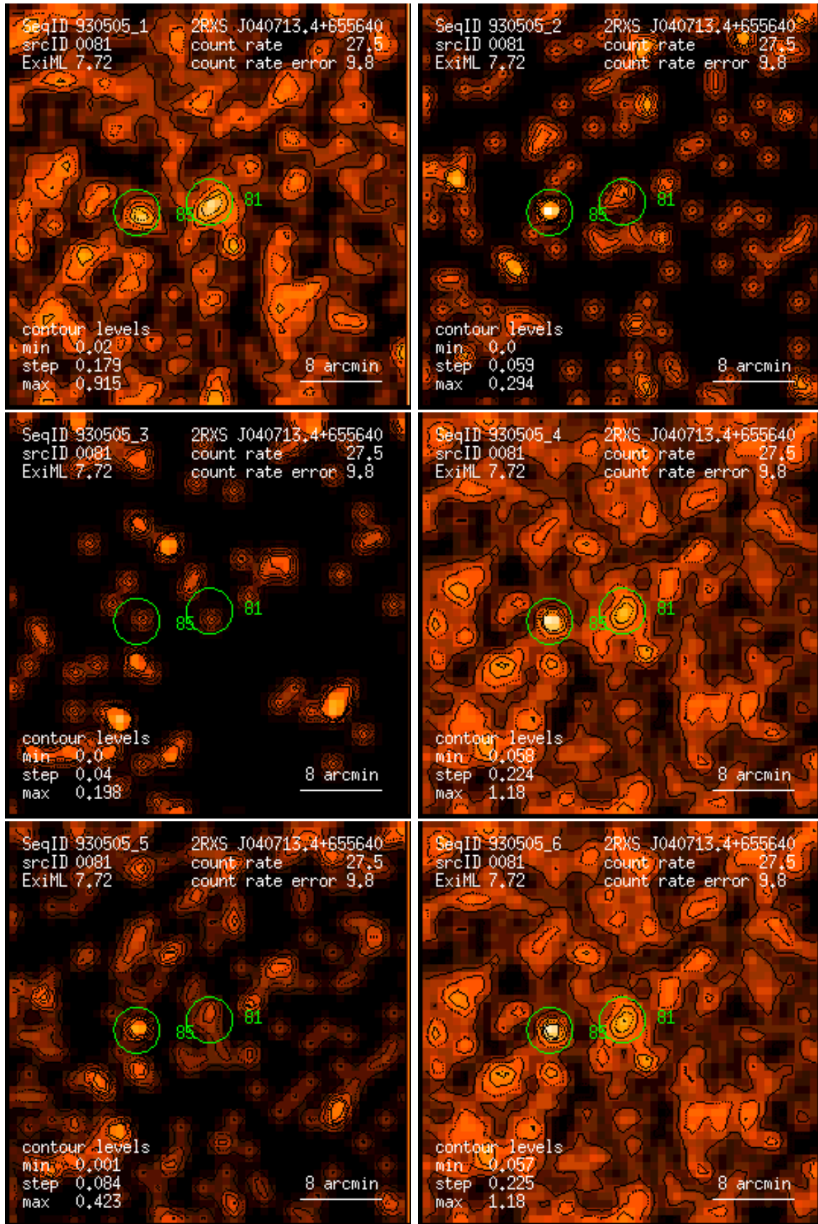
Figure 81: RASS 930505: detection 0081: band rate images, Gaussian filter: (1) PSPC channels 11 – 41, (2) 52 – 90, (3) 91 – 201, (4) 11 – 235, (5) 52 – 201, (6) 11 – 201. Broad band rates in counts/ks. Band rate contour levels in counts/ks/arcmin 2 .
