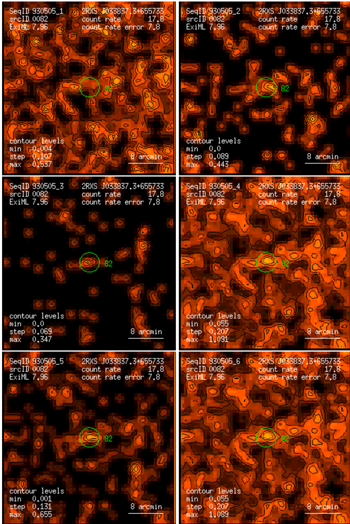
Figure 82: RASS 930505: detection 0082: band rate images, Gaussian filter: (1) PSPC channels 11 – 41, (2) 52 – 90, (3) 91 – 201, (4) 11 – 235, (5) 52 – 201, (6) 11 – 201. Broad band rates in counts/ks. Band rate contour levels in counts/ks/arcmin 2 .
