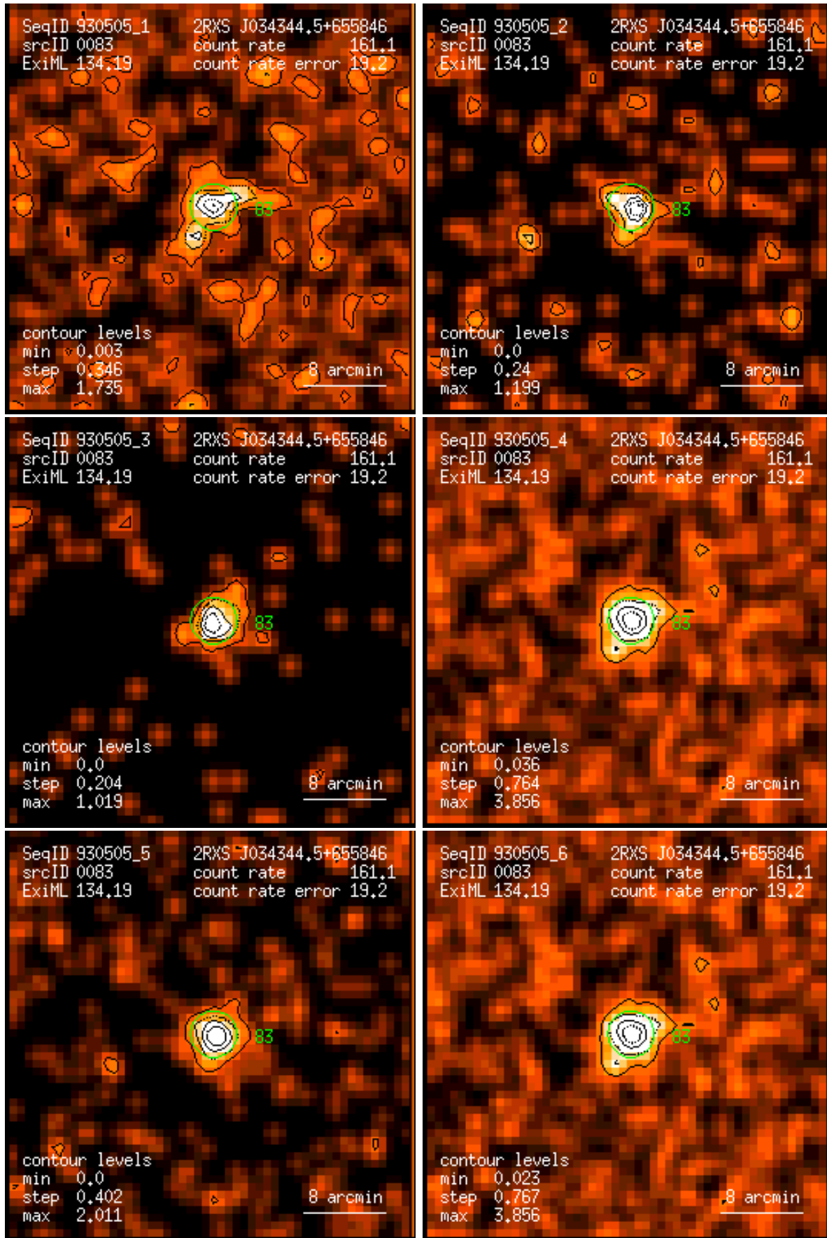
Figure 83: RASS 930505: detection 0083: band rate images, Gaussian filter: (1) PSPC channels 11 – 41, (2) 52 – 90, (3) 91 – 201, (4) 11 – 235, (5) 52 – 201, (6) 11 – 201. Broad band rates in counts/ks. Band rate contour levels in counts/ks/arcmin 2 .
