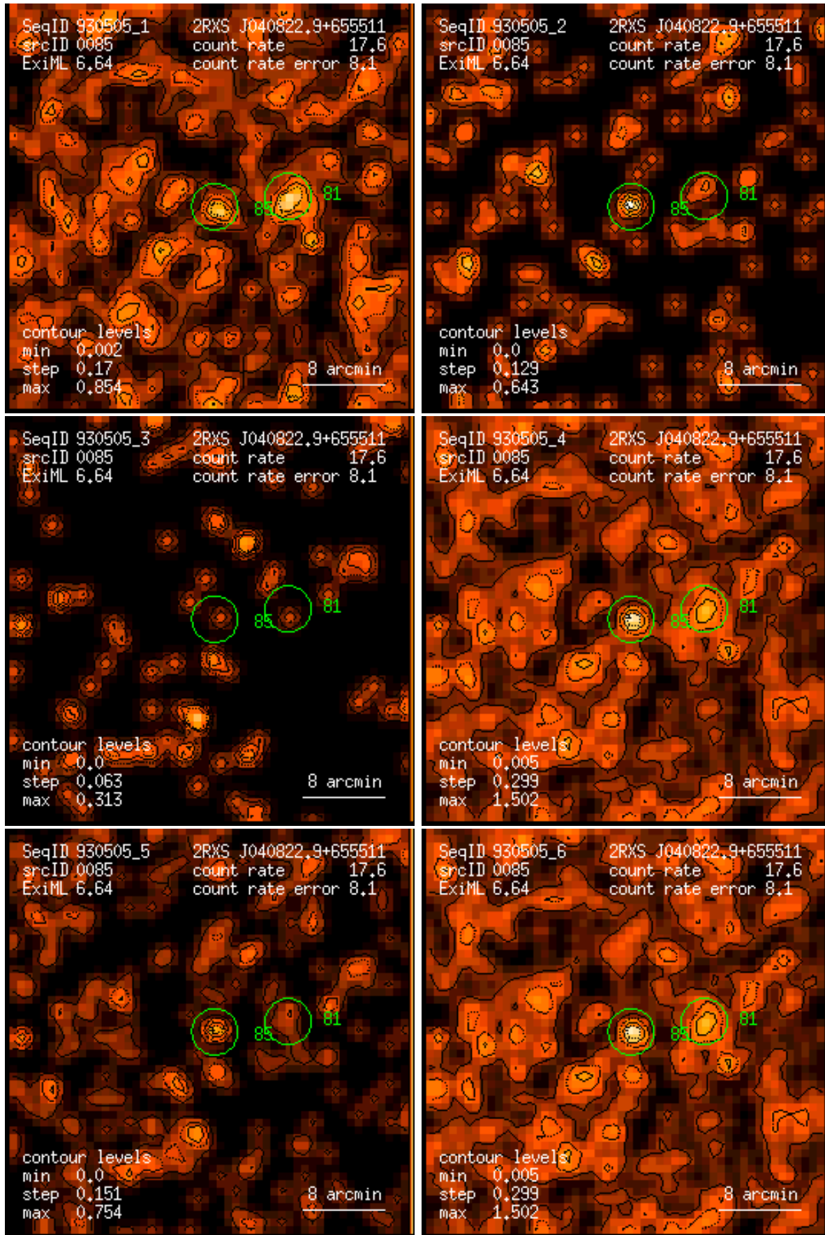
Figure 85: RASS 930505: detection 0085: band rate images, Gaussian filter: (1) PSPC channels 11 – 41, (2) 52 – 90, (3) 91 – 201, (4) 11 – 235, (5) 52 – 201, (6) 11 – 201. Broad band rates in counts/ks. Band rate contour levels in counts/ks/arcmin 2 .
