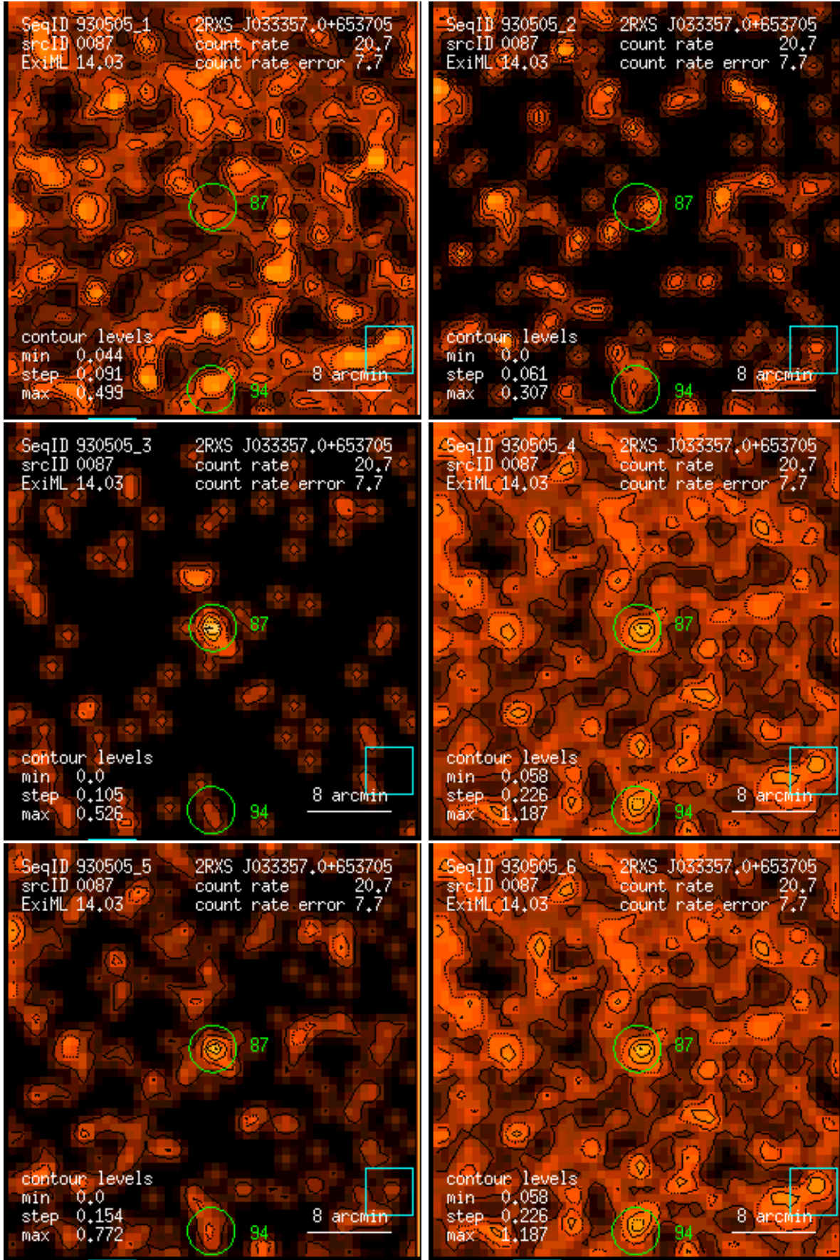
Figure 87: RASS 930505: detection 0087: band rate images, Gaussian filter: (1) PSPC channels 11 – 41, (2) 52 – 90, (3) 91 – 201, (4) 11 – 235, (5) 52 – 201, (6) 11 – 201. Broad band rates in counts/ks. Band rate contour levels in counts/ks/arcmin 2 .
