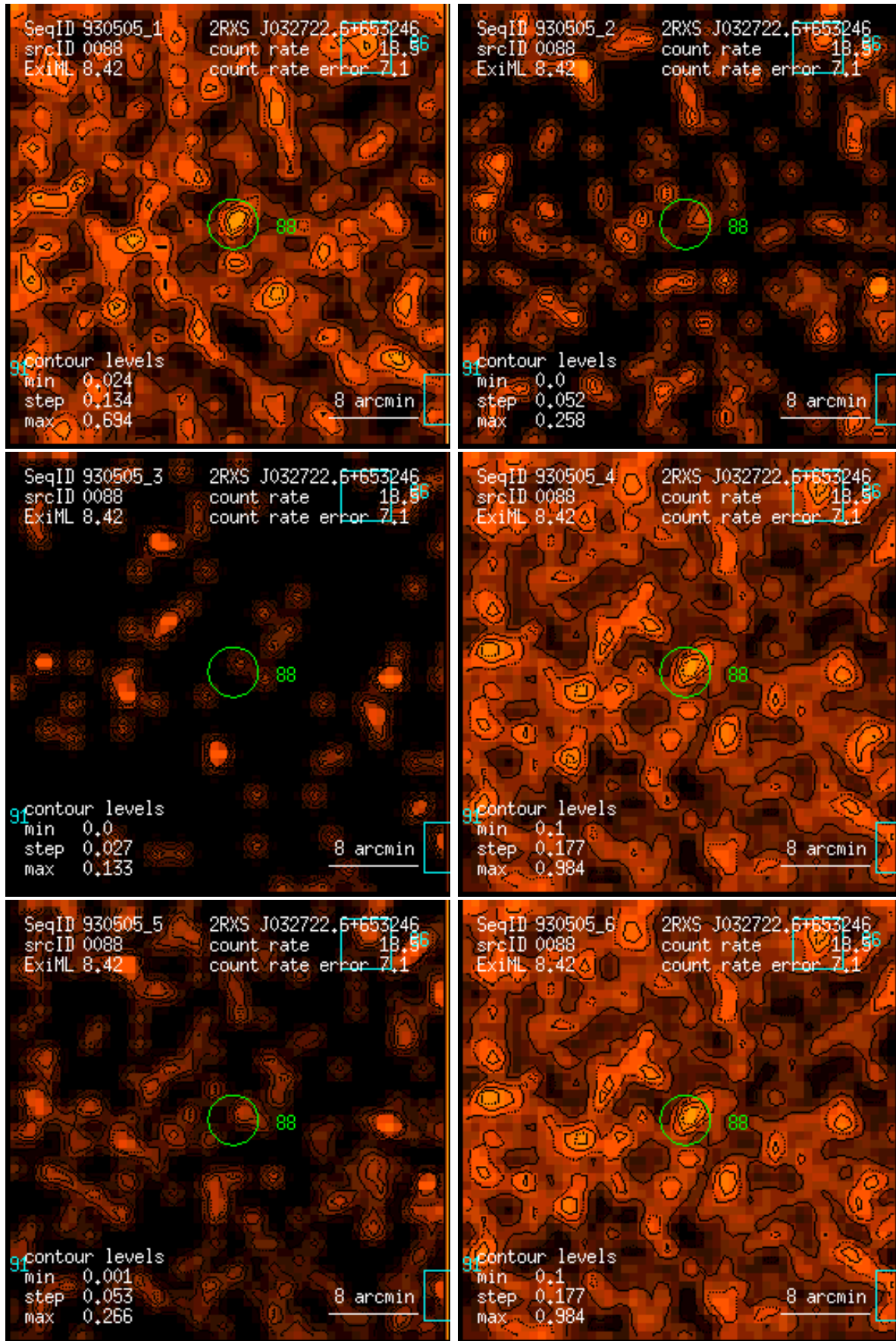
Figure 88: RASS 930505: detection 0088: band rate images, Gaussian filter: (1) PSPC channels 11 – 41, (2) 52 – 90, (3) 91 – 201, (4) 11 – 235, (5) 52 – 201, (6) 11 – 201. Broad band rates in counts/ks. Band rate contour levels in counts/ks/arcmin 2 .
