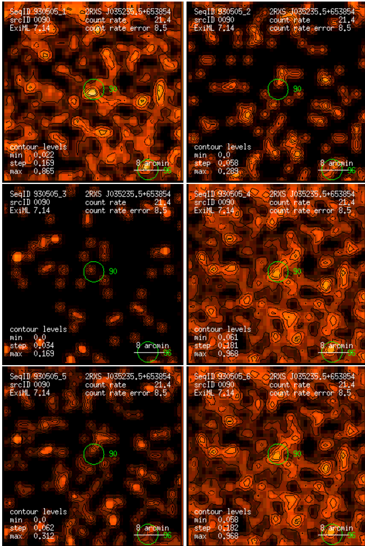
Figure 90: RASS 930505: detection 0090: band rate images, Gaussian filter: (1) PSPC channels 11 – 41, (2) 52 – 90, (3) 91 – 201, (4) 11 – 235, (5) 52 – 201, (6) 11 – 201. Broad band rates in counts/ks. Band rate contour levels in counts/ks/arcmin 2 .
