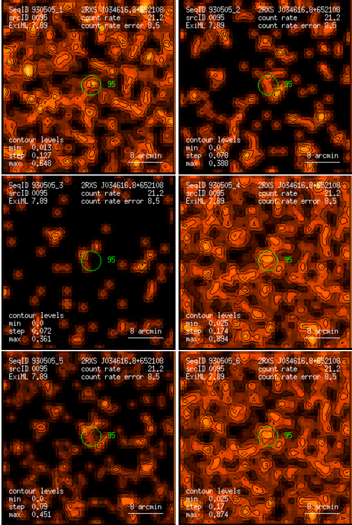
Figure 95: RASS 930505: detection 0095: band rate images, Gaussian filter: (1) PSPC channels 11 – 41, (2) 52 – 90, (3) 91 – 201, (4) 11 – 235, (5) 52 – 201, (6) 11 – 201. Broad band rates in counts/ks. Band rate contour levels in counts/ks/arcmin 2 .
