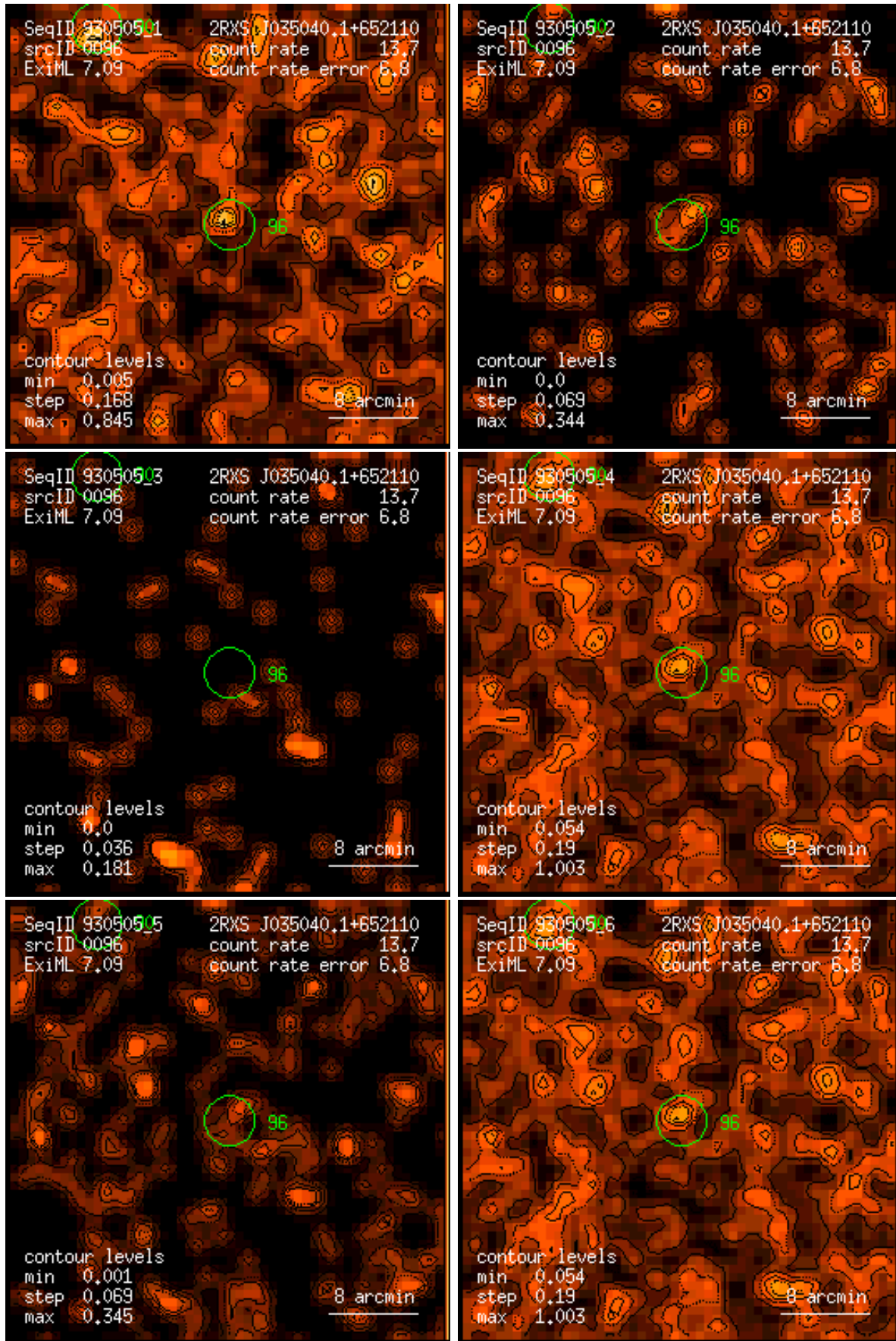
Figure 96: RASS 930505: detection 0096: band rate images, Gaussian filter: (1) PSPC channels 11 – 41, (2) 52 – 90, (3) 91 – 201, (4) 11 – 235, (5) 52 – 201, (6) 11 – 201. Broad band rates in counts/ks. Band rate contour levels in counts/ks/arcmin 2 .
