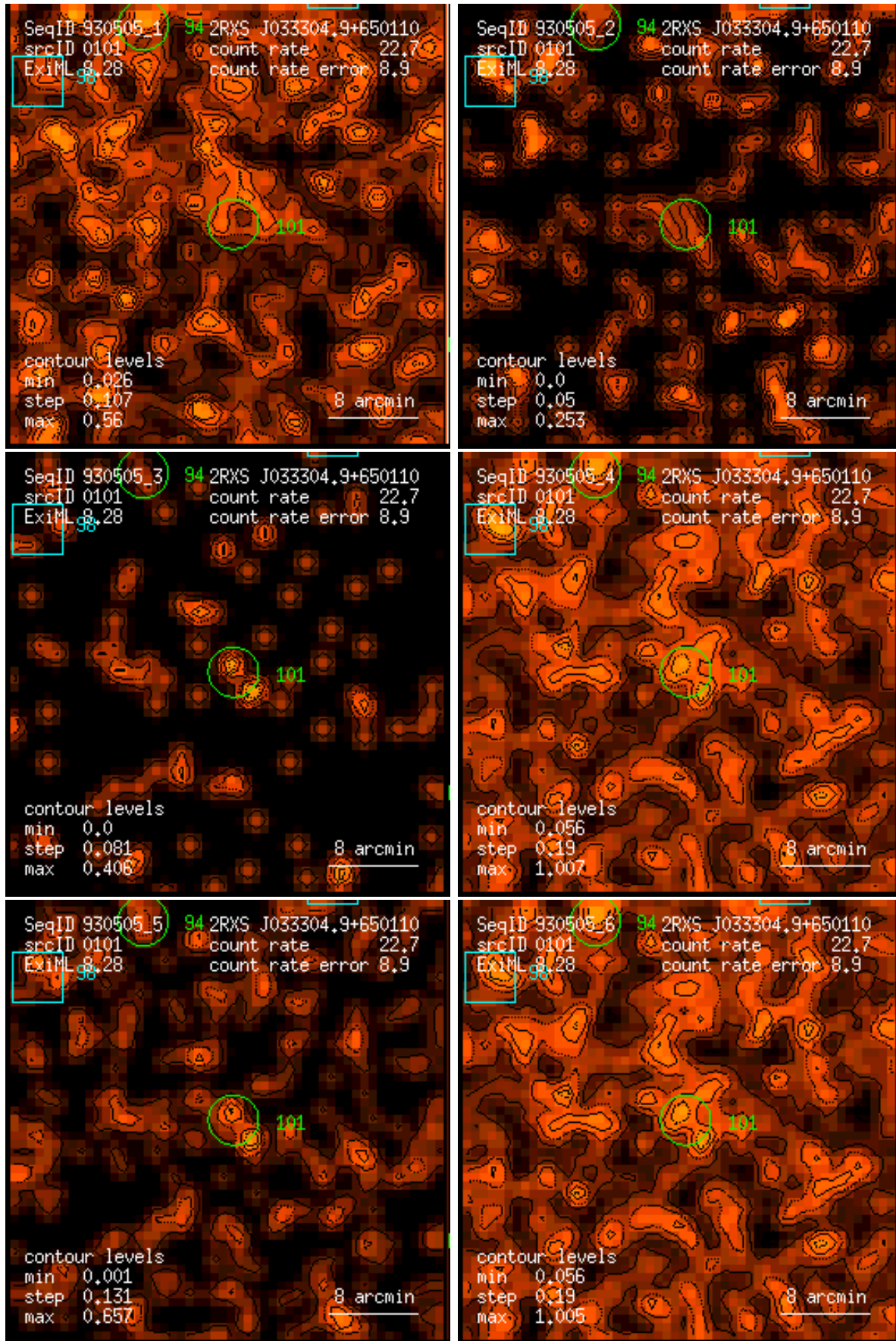
Figure 101: RASS 930505: detection 0101: band rate images, Gaussian filter: (1) PSPC channels 11 – 41, (2) 52 – 90, (3) 91 – 201, (4) 11 – 235, (5) 52 – 201, (6) 11 – 201. Broad band rates in counts/ks. Band rate contour levels in counts/ks/arcmin 2 .
