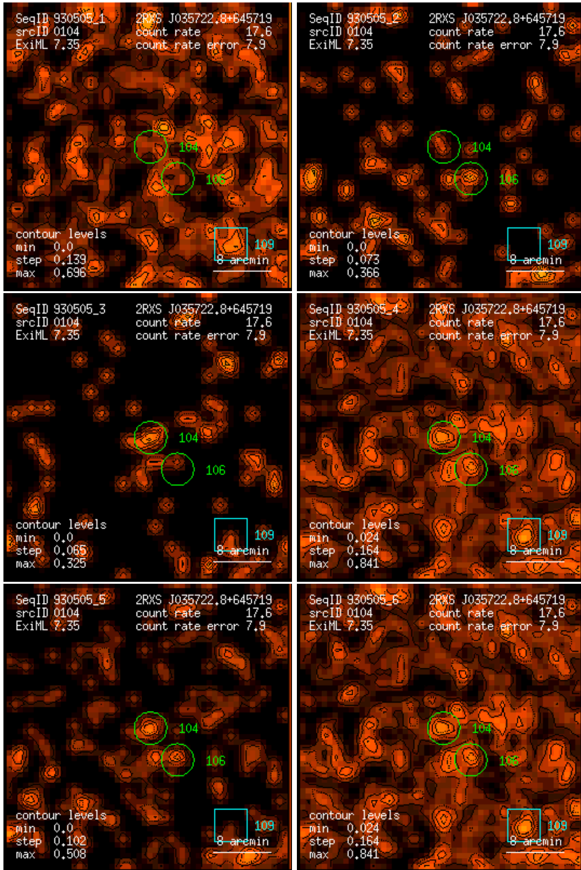
Figure 104: RASS 930505: detection 0104: band rate images, Gaussian filter: (1) PSPC channels 11 – 41, (2) 52 – 90, (3) 91 – 201, (4) 11 – 235, (5) 52 – 201, (6) 11 – 201. Broad band rates in counts/ks. Band rate contour levels in counts/ks/arcmin 2 .
