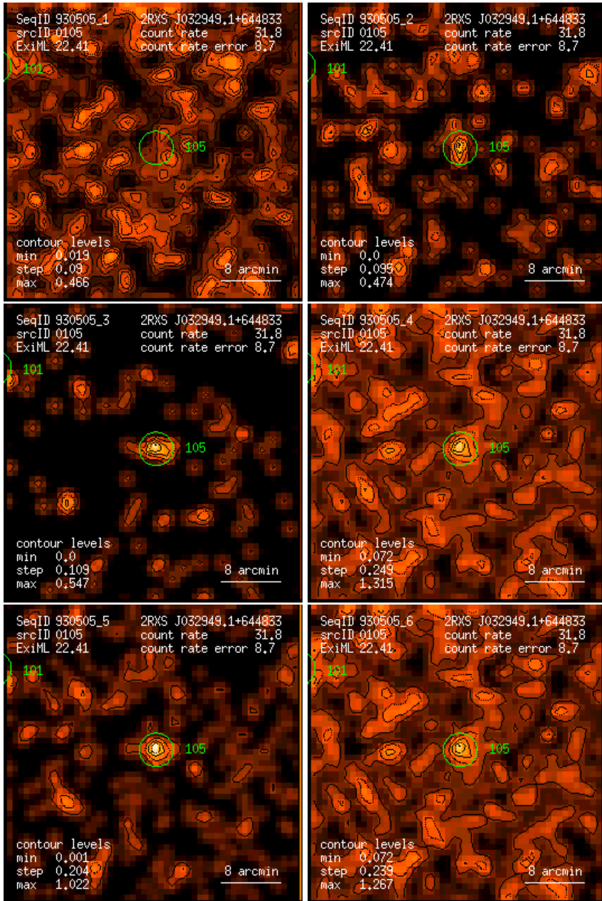
Figure 105: RASS 930505: detection 0105: band rate images, Gaussian filter: (1) PSPC channels 11 – 41, (2) 52 – 90, (3) 91 – 201, (4) 11 – 235, (5) 52 – 201, (6) 11 – 201. Broad band rates in counts/ks. Band rate contour levels in counts/ks/arcmin 2 .
