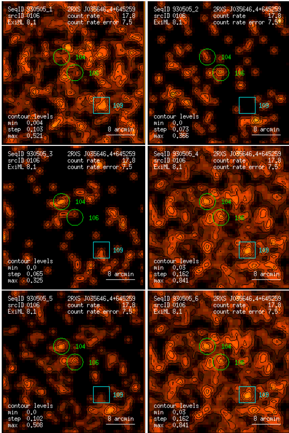
Figure 106: RASS 930505: detection 0106: band rate images, Gaussian filter: (1) PSPC channels 11 – 41, (2) 52 – 90, (3) 91 – 201, (4) 11 – 235, (5) 52 – 201, (6) 11 – 201. Broad band rates in counts/ks. Band rate contour levels in counts/ks/arcmin 2 .
