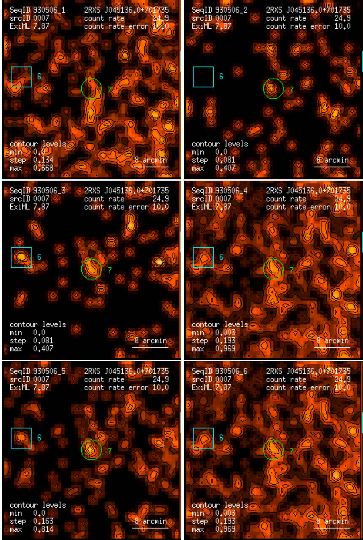
Figure 7: RASS 930506: detection 0007: band rate images, Gaussian filter: (1) PSPC channels 11 – 41, (2) 52 – 90, (3) 91 – 201, (4) 11 – 235, (5) 52 – 201, (6) 11 – 201. Broad band rates in counts/ks. Band rate contour levels in counts/ks/arcmin 2 .
