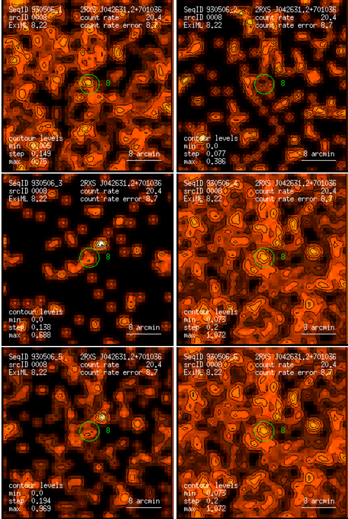
Figure 8: RASS 930506: detection 0008: band rate images, Gaussian filter: (1) PSPC channels 11 – 41, (2) 52 – 90, (3) 91 – 201, (4) 11 – 235, (5) 52 – 201, (6) 11 – 201. Broad band rates in counts/ks. Band rate contour levels in counts/ks/arcmin 2 .
