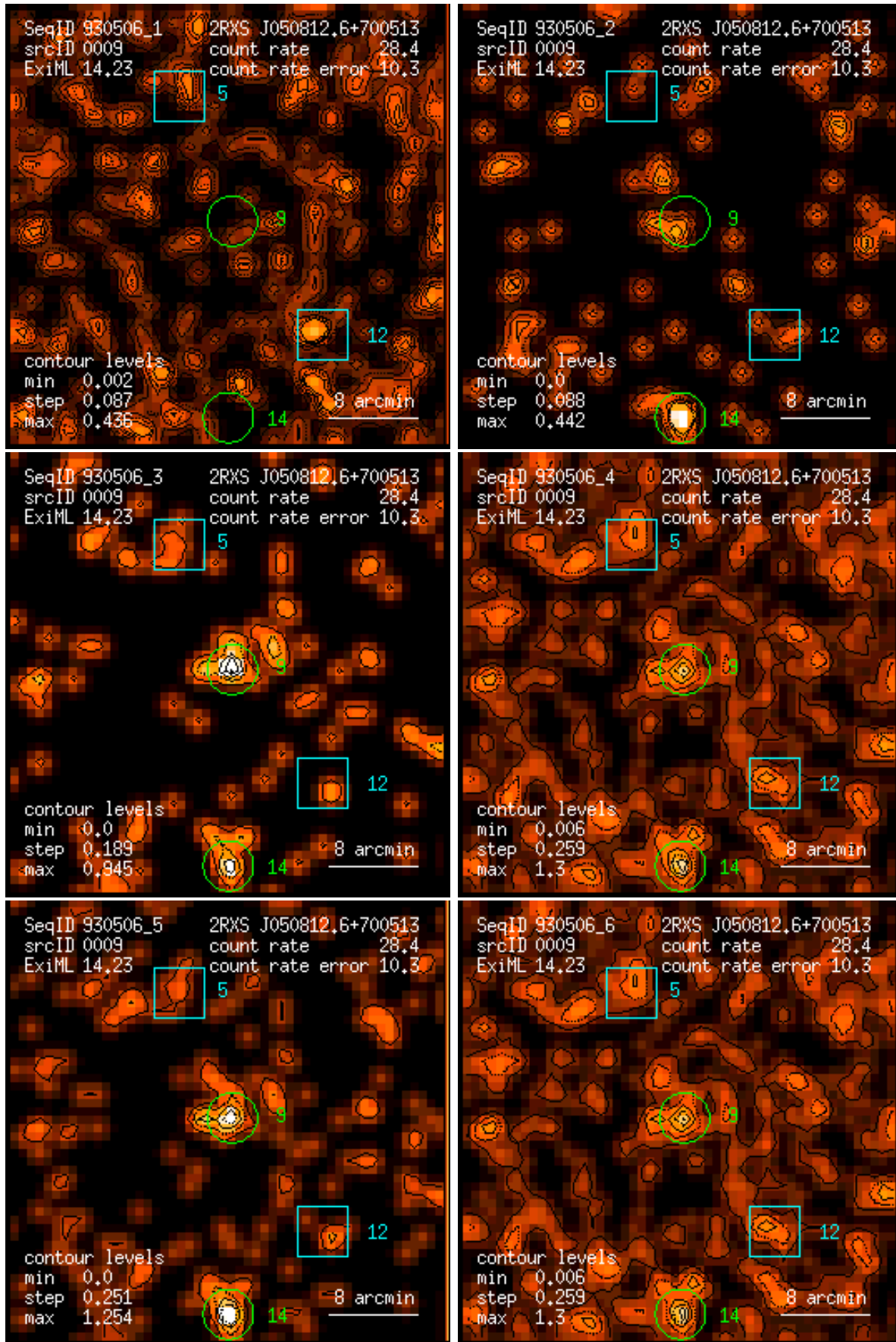
Figure 9: RASS 930506: detection 0009: band rate images, Gaussian filter: (1) PSPC channels 11 – 41, (2) 52 – 90, (3) 91 – 201, (4) 11 – 235, (5) 52 – 201, (6) 11 – 201. Broad band rates in counts/ks. Band rate contour levels in counts/ks/arcmin 2 .
