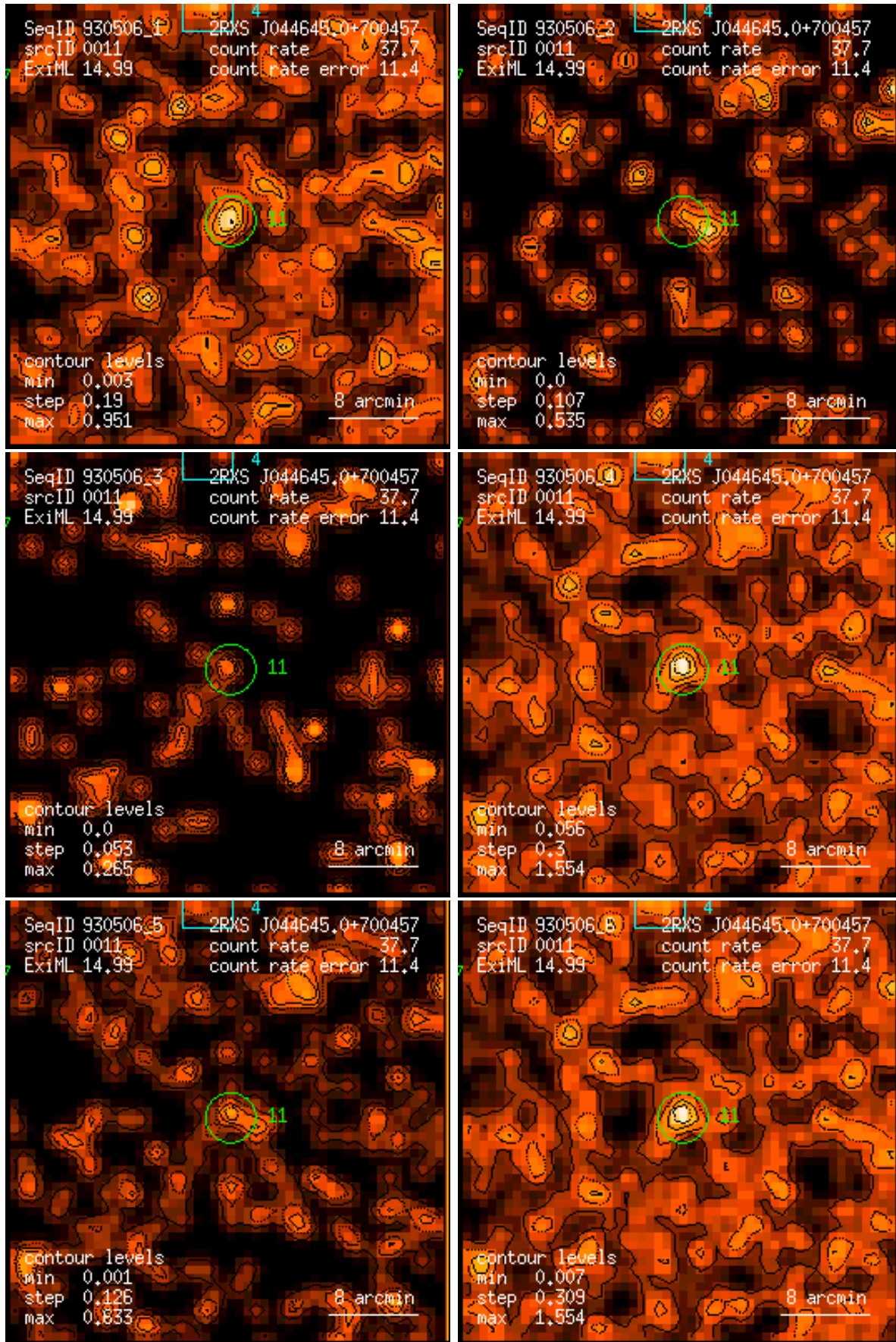
Figure 11: RASS 930506: detection 0011: band rate images, Gaussian filter: (1) PSPC channels 11 – 41, (2) 52 – 90, (3) 91 – 201, (4) 11 – 235, (5) 52 – 201, (6) 11 – 201. Broad band rates in counts/ks. Band rate contour levels in counts/ks/arcmin 2 .
