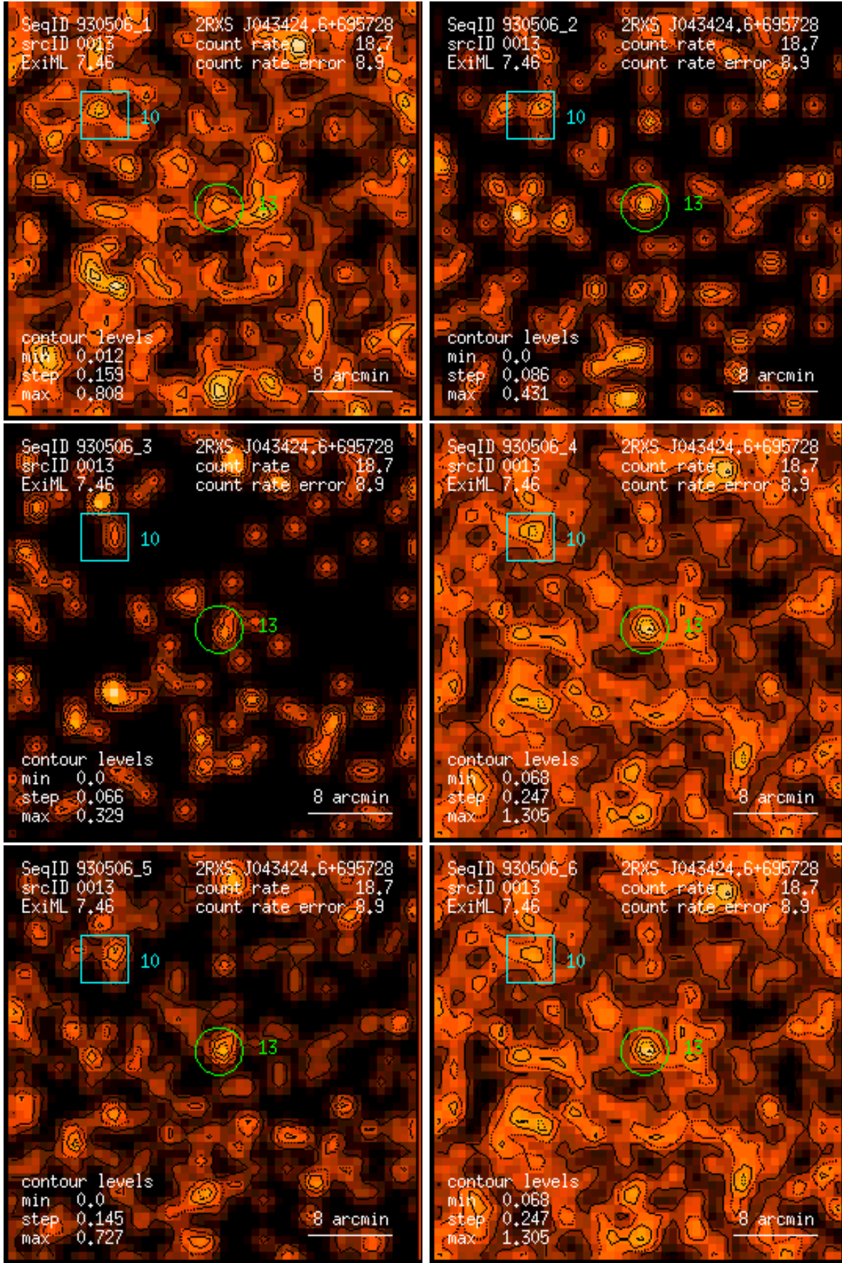
Figure 13: RASS 930506: detection 0013: band rate images, Gaussian filter: (1) PSPC channels 11 – 41, (2) 52 – 90, (3) 91 – 201, (4) 11 – 235, (5) 52 – 201, (6) 11 – 201. Broad band rates in counts/ks. Band rate contour levels in counts/ks/arcmin 2 .
