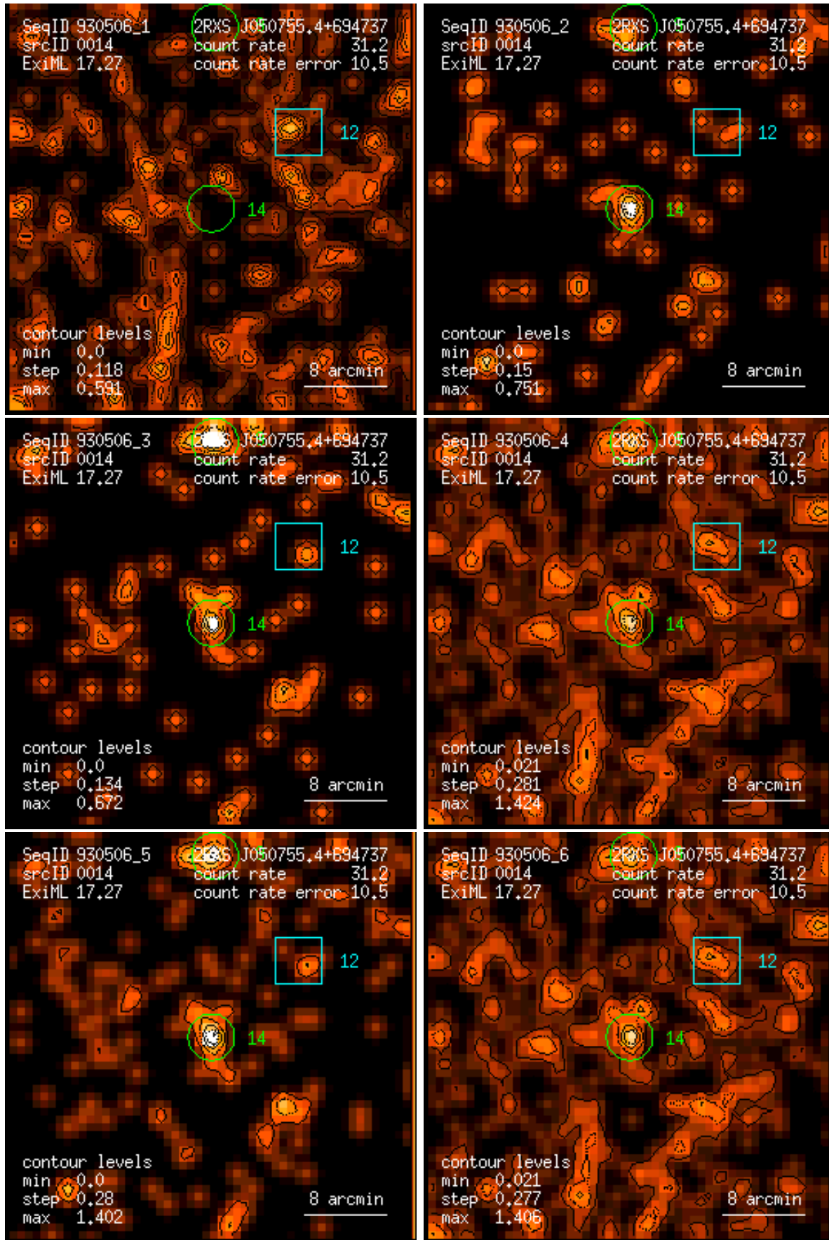
Figure 14: RASS 930506: detection 0014: band rate images, Gaussian filter: (1) PSPC channels 11 – 41, (2) 52 – 90, (3) 91 – 201, (4) 11 – 235, (5) 52 – 201, (6) 11 – 201. Broad band rates in counts/ks. Band rate contour levels in counts/ks/arcmin 2 .
