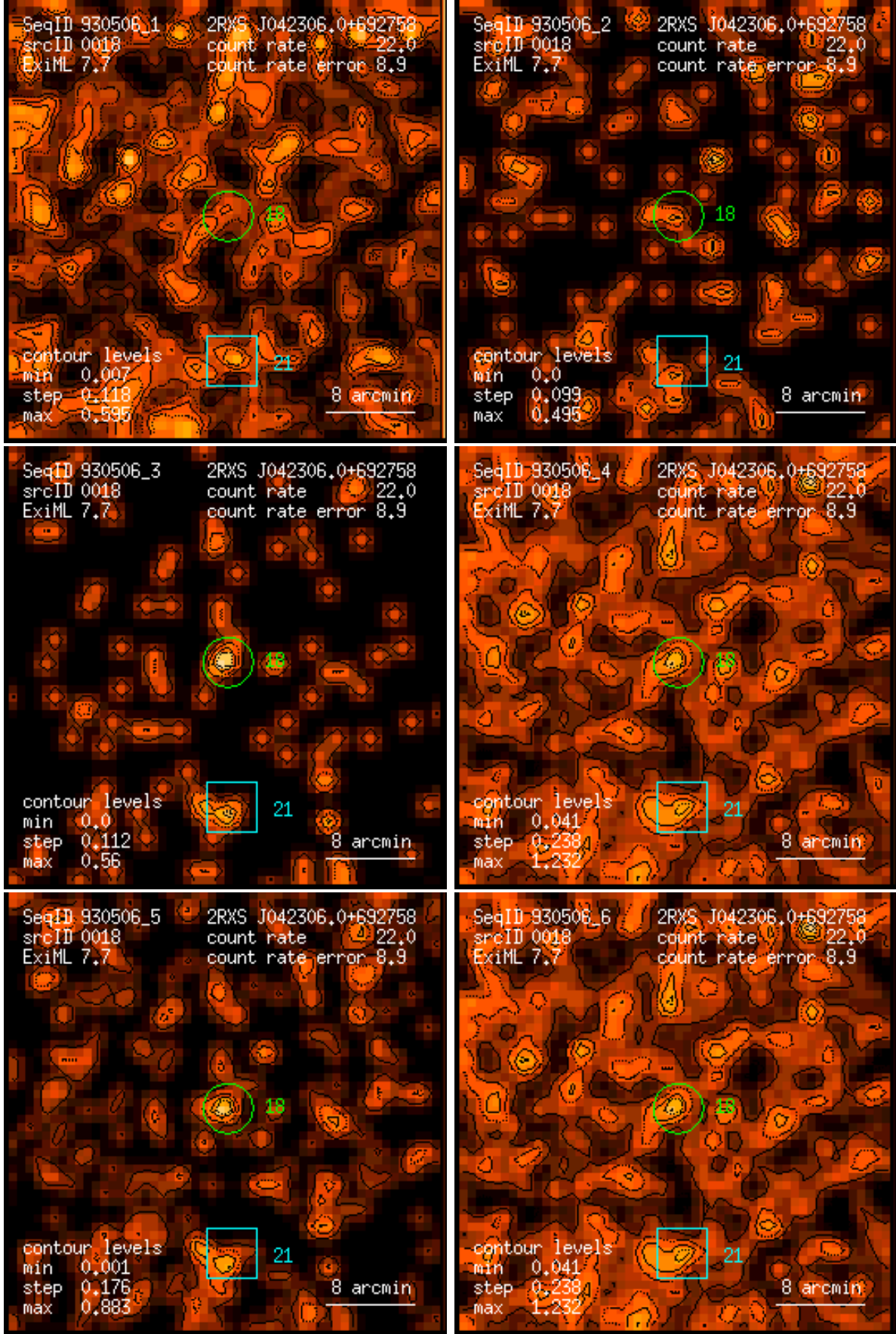
Figure 18: RASS 930506: detection 0018: band rate images, Gaussian filter: (1) PSPC channels 11 – 41, (2) 52 – 90, (3) 91 – 201, (4) 11 – 235, (5) 52 – 201, (6) 11 – 201. Broad band rates in counts/ks. Band rate contour levels in counts/ks/arcmin 2 .
