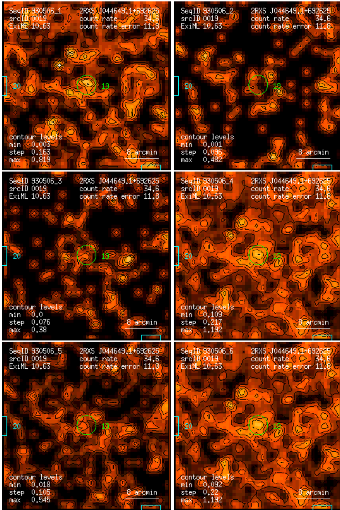
Figure 19: RASS 930506: detection 0019: band rate images, Gaussian filter: (1) PSPC channels 11 – 41, (2) 52 – 90, (3) 91 – 201, (4) 11 – 235, (5) 52 – 201, (6) 11 – 201. Broad band rates in counts/ks. Band rate contour levels in counts/ks/arcmin 2 .
