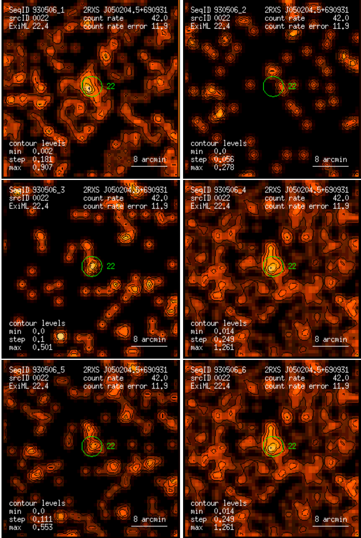
Figure 22: RASS 930506: detection 0022: band rate images, Gaussian filter: (1) PSPC channels 11 – 41, (2) 52 – 90, (3) 91 – 201, (4) 11 – 235, (5) 52 – 201, (6) 11 – 201. Broad band rates in counts/ks. Band rate contour levels in counts/ks/arcmin 2 .
