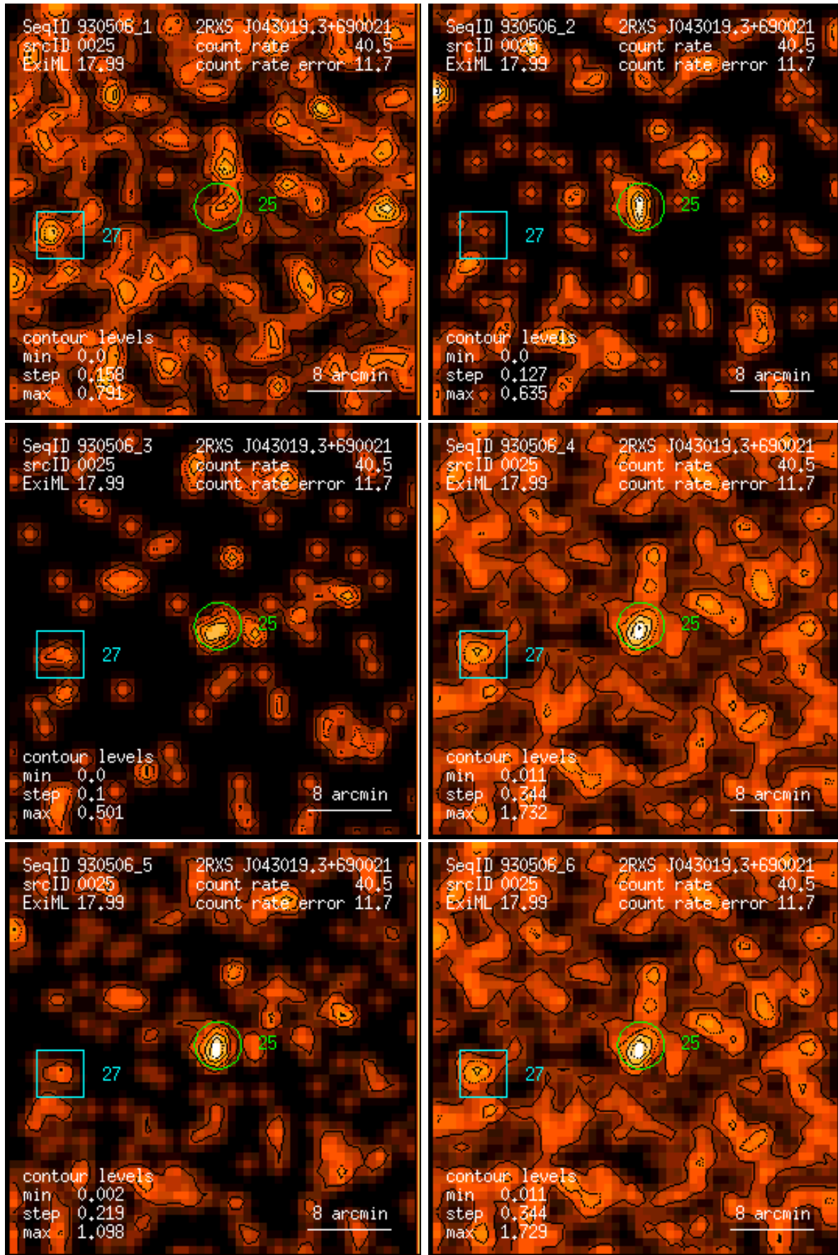
Figure 25: RASS 930506: detection 0025: band rate images, Gaussian filter: (1) PSPC channels 11 – 41, (2) 52 – 90, (3) 91 – 201, (4) 11 – 235, (5) 52 – 201, (6) 11 – 201. Broad band rates in counts/ks. Band rate contour levels in counts/ks/arcmin 2 .
