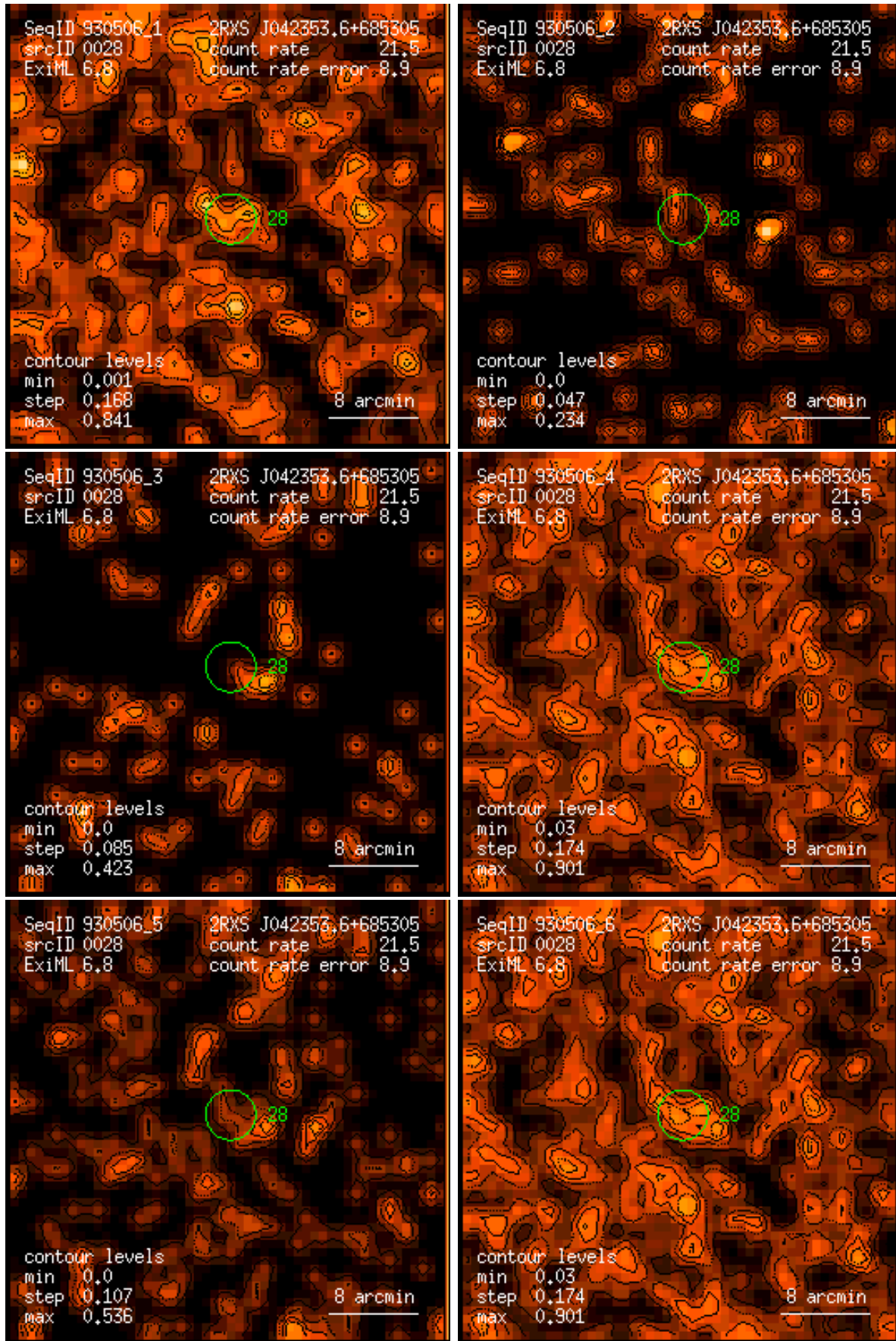
Figure 28: RASS 930506: detection 0028: band rate images, Gaussian filter: (1) PSPC channels 11 – 41, (2) 52 – 90, (3) 91 – 201, (4) 11 – 235, (5) 52 – 201, (6) 11 – 201. Broad band rates in counts/ks. Band rate contour levels in counts/ks/arcmin 2 .
