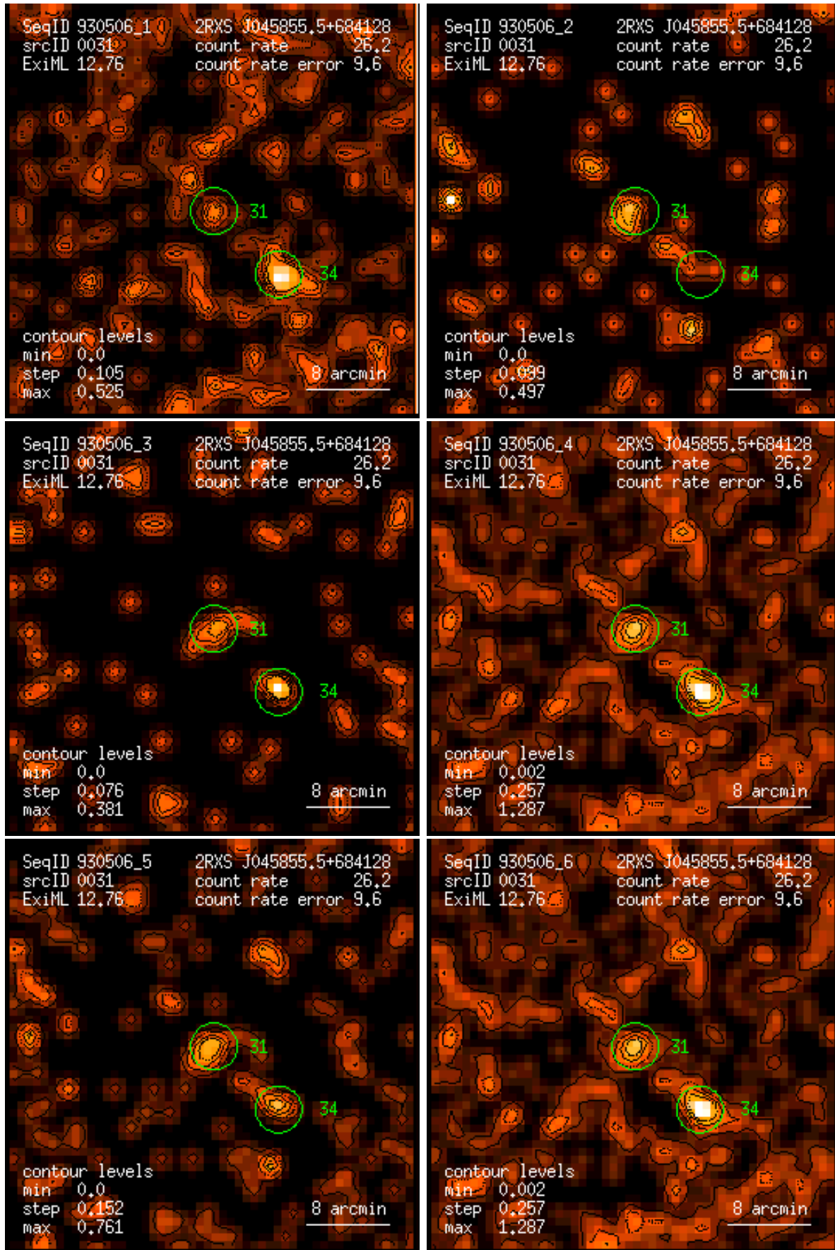
Figure 31: RASS 930506: detection 0031: band rate images, Gaussian filter: (1) PSPC channels 11 – 41, (2) 52 – 90, (3) 91 – 201, (4) 11 – 235, (5) 52 – 201, (6) 11 – 201. Broad band rates in counts/ks. Band rate contour levels in counts/ks/arcmin 2 .
