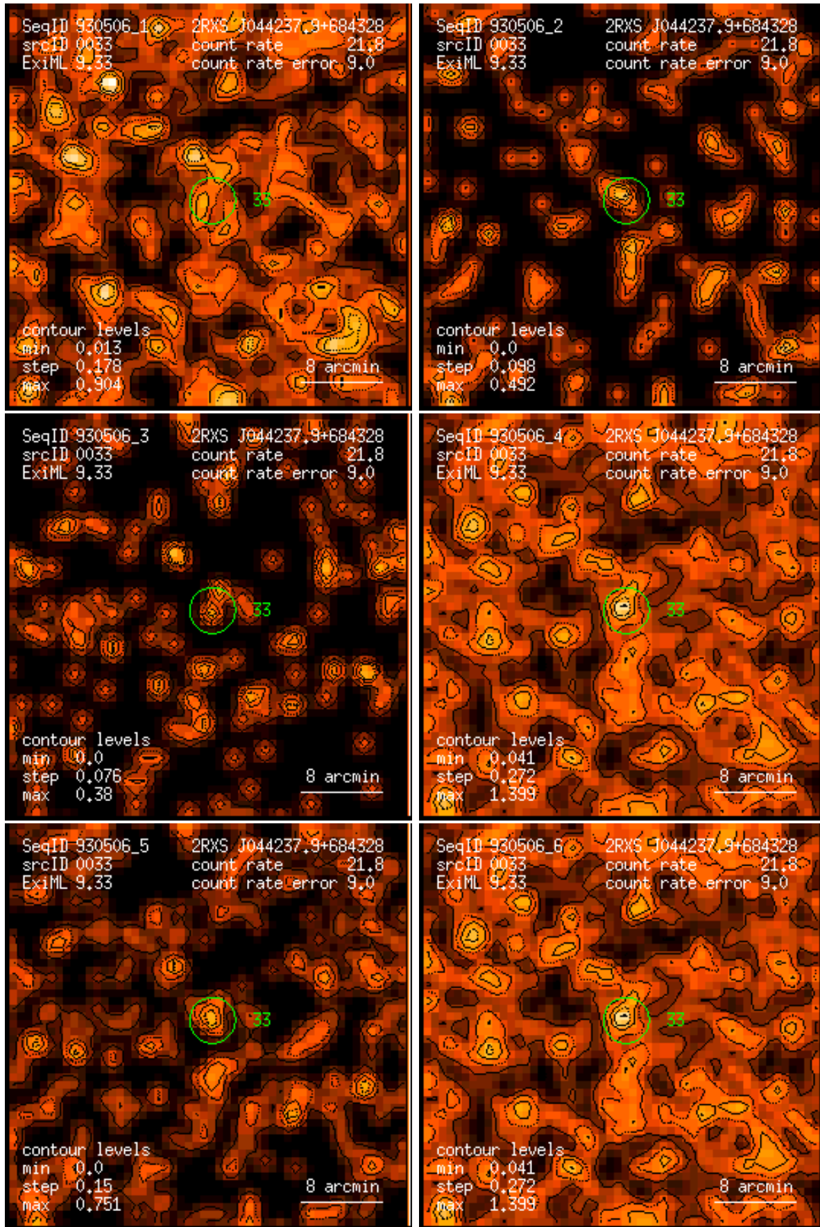
Figure 33: RASS 930506: detection 0033: band rate images, Gaussian filter: (1) PSPC channels 11 – 41, (2) 52 – 90, (3) 91 – 201, (4) 11 – 235, (5) 52 – 201, (6) 11 – 201. Broad band rates in counts/ks. Band rate contour levels in counts/ks/arcmin 2 .
