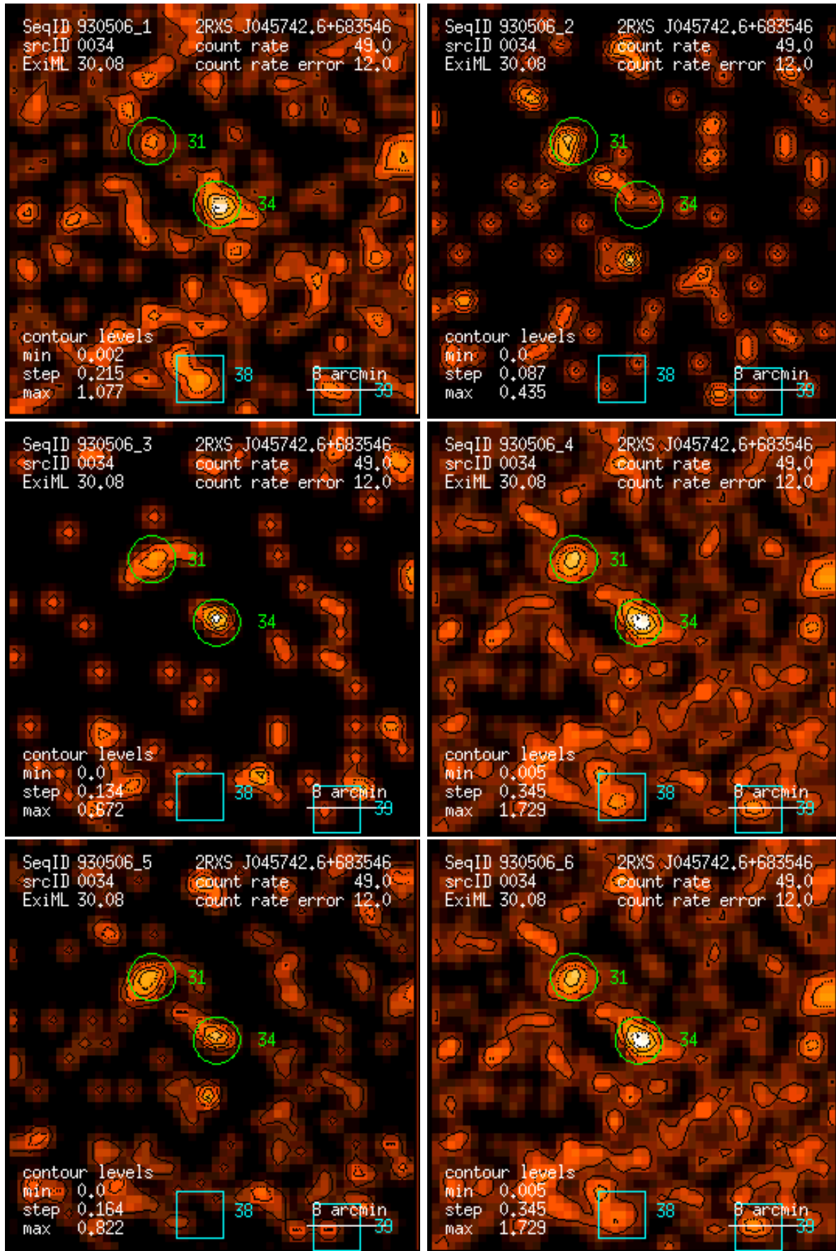
Figure 34: RASS 930506: detection 0034: band rate images, Gaussian filter: (1) PSPC channels 11 – 41, (2) 52 – 90, (3) 91 – 201, (4) 11 – 235, (5) 52 – 201, (6) 11 – 201. Broad band rates in counts/ks. Band rate contour levels in counts/ks/arcmin 2 .
