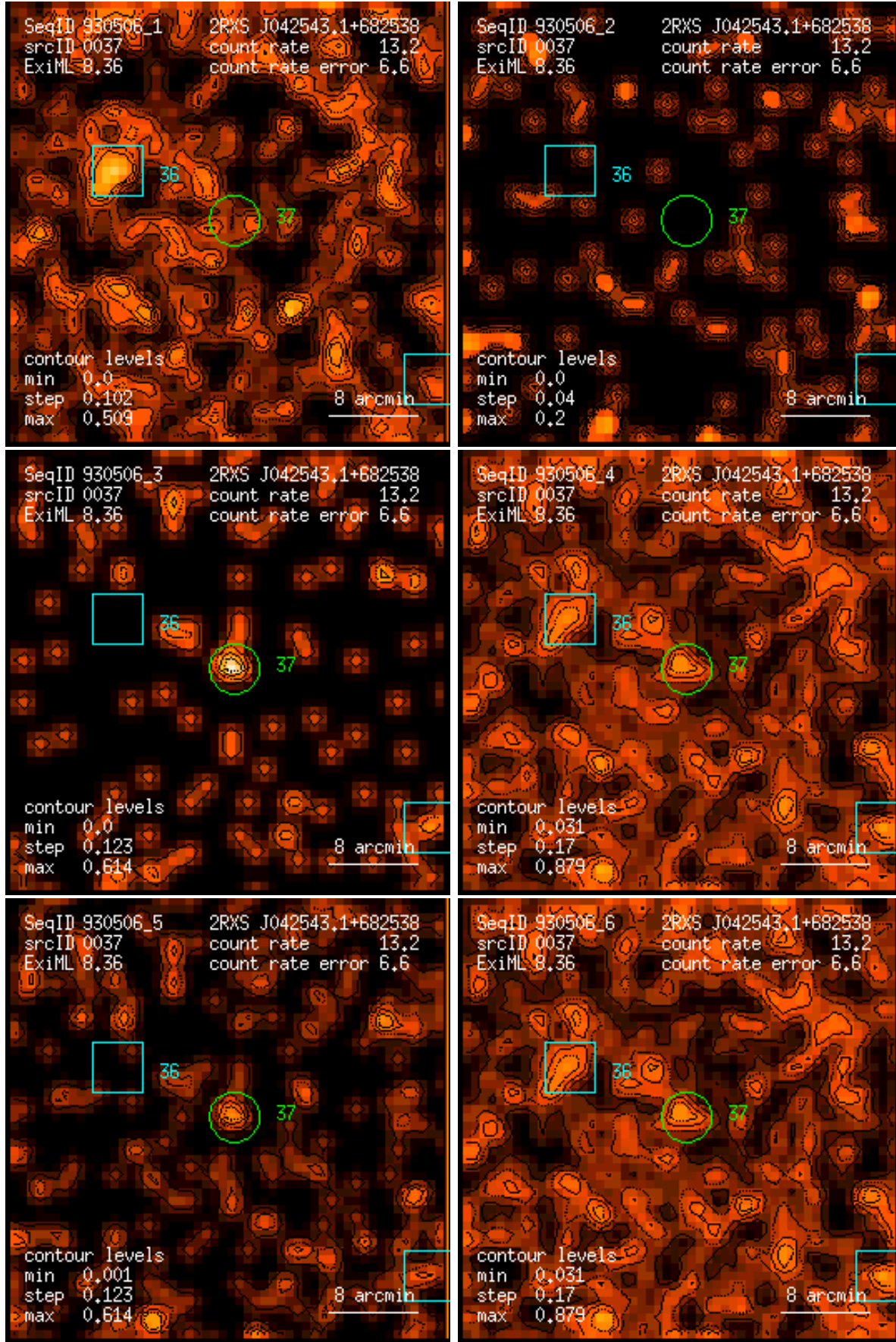
Figure 37: RASS 930506: detection 0037: band rate images, Gaussian filter: (1) PSPC channels 11 – 41, (2) 52 – 90, (3) 91 – 201, (4) 11 – 235, (5) 52 – 201, (6) 11 – 201. Broad band rates in counts/ks. Band rate contour levels in counts/ks/arcmin 2 .
