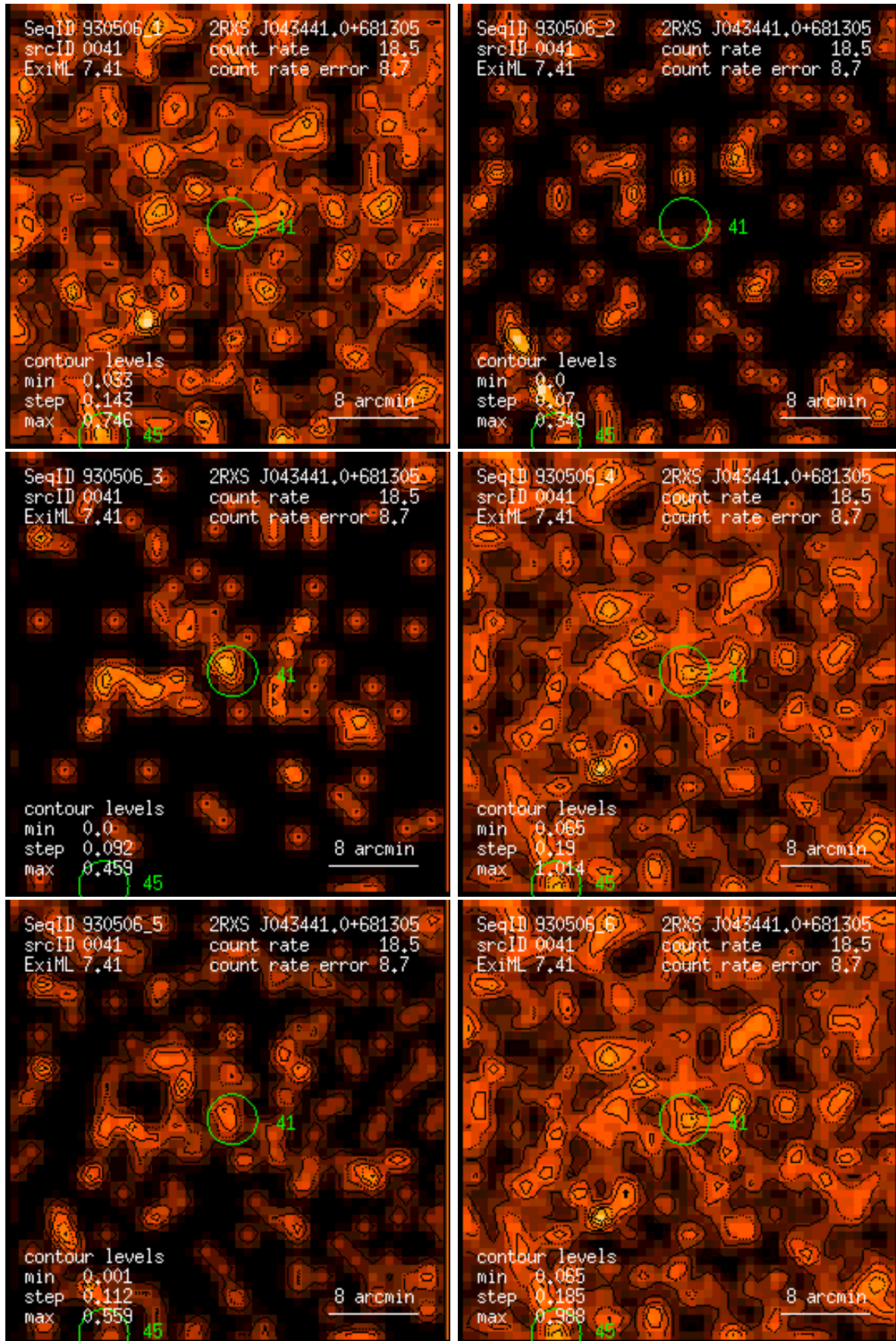
Figure 41: RASS 930506: detection 0041: band rate images, Gaussian filter: (1) PSPC channels 11 – 41, (2) 52 – 90, (3) 91 – 201, (4) 11 – 235, (5) 52 – 201, (6) 11 – 201. Broad band rates in counts/ks. Band rate contour levels in counts/ks/arcmin 2 .
