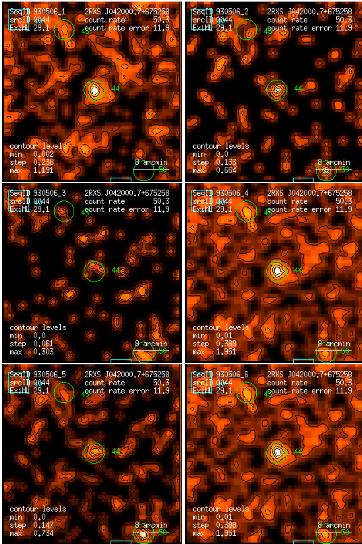
Figure 44: RASS 930506: detection 0044: band rate images, Gaussian filter: (1) PSPC channels 11 – 41, (2) 52 – 90, (3) 91 – 201, (4) 11 – 235, (5) 52 – 201, (6) 11 – 201. Broad band rates in counts/ks. Band rate contour levels in counts/ks/arcmin 2 .
