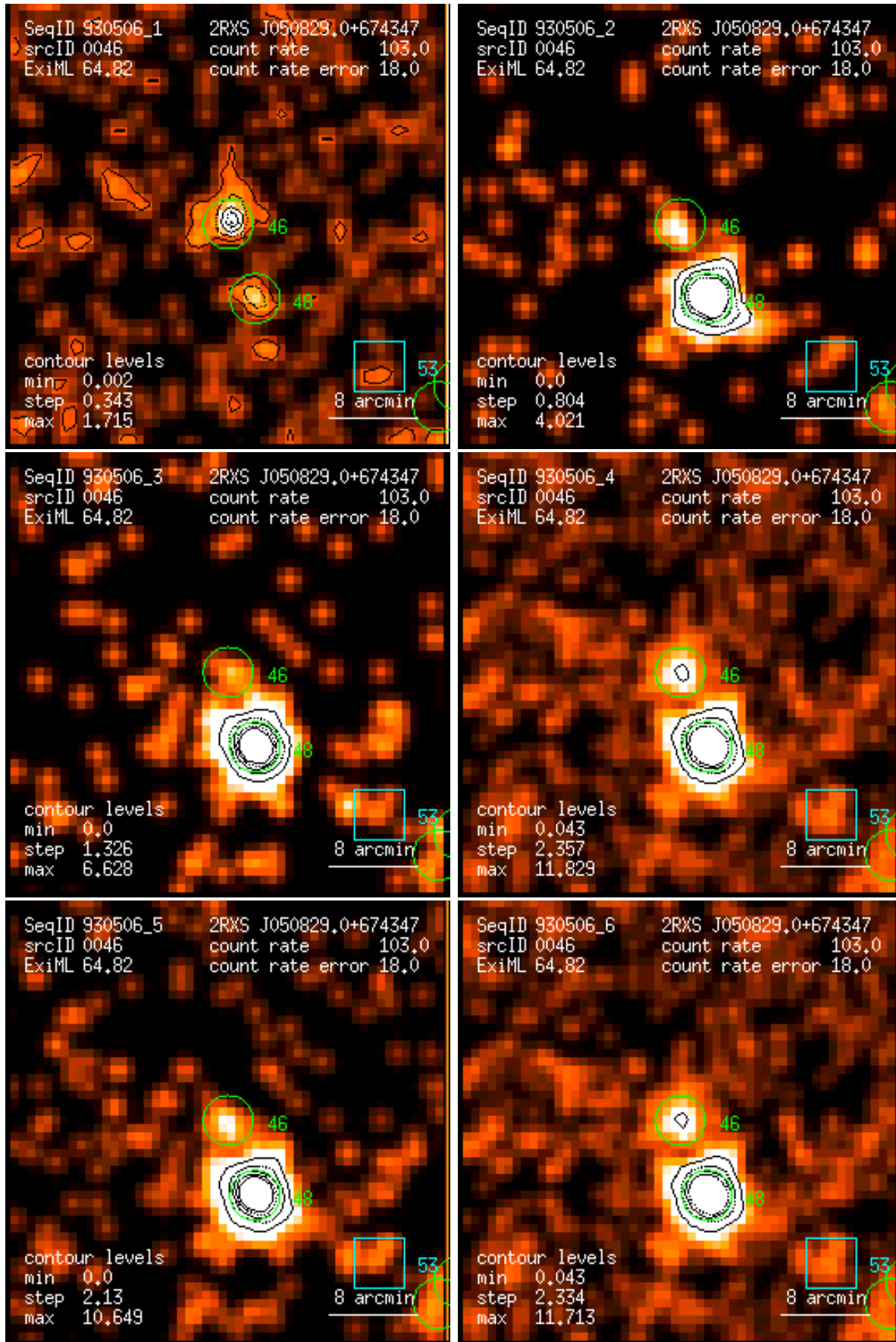
Figure 46: RASS 930506: detection 0046: band rate images, Gaussian filter: (1) PSPC channels 11 – 41, (2) 52 – 90, (3) 91 – 201, (4) 11 – 235, (5) 52 – 201, (6) 11 – 201. Broad band rates in counts/ks. Band rate contour levels in counts/ks/arcmin 2 .
