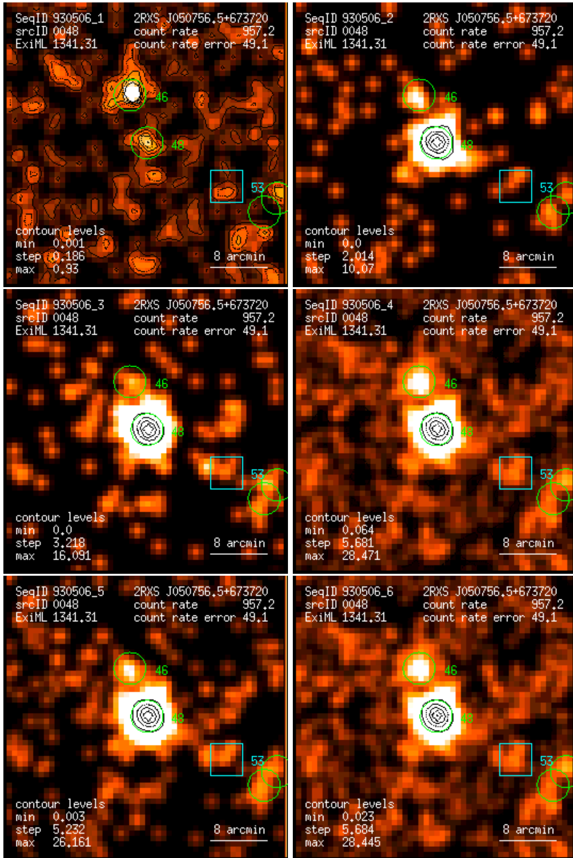
Figure 48: RASS 930506: detection 0048: band rate images, Gaussian filter: (1) PSPC channels 11 – 41, (2) 52 – 90, (3) 91 – 201, (4) 11 – 235, (5) 52 – 201, (6) 11 – 201. Broad band rates in counts/ks. Band rate contour levels in counts/ks/arcmin 2 .
