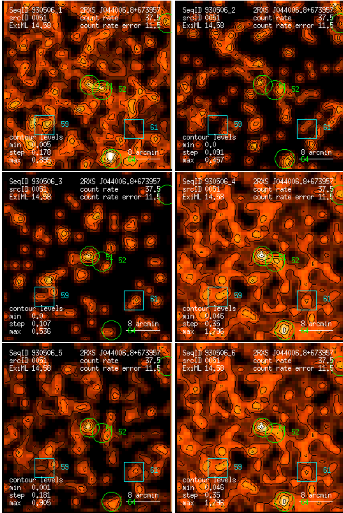
Figure 51: RASS 930506: detection 0051: band rate images, Gaussian filter: (1) PSPC channels 11 – 41, (2) 52 – 90, (3) 91 – 201, (4) 11 – 235, (5) 52 – 201, (6) 11 – 201. Broad band rates in counts/ks. Band rate contour levels in counts/ks/arcmin 2 .
