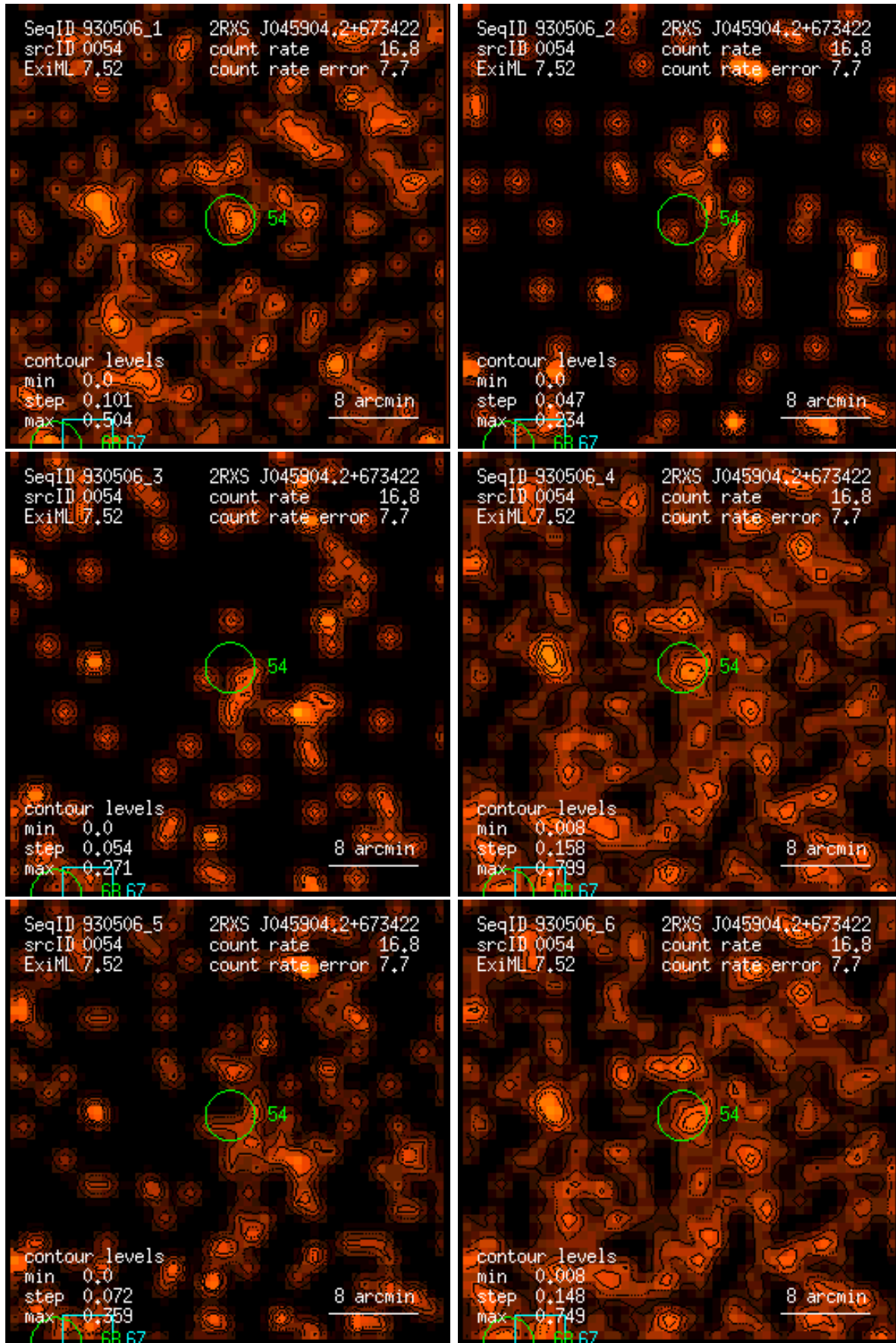
Figure 54: RASS 930506: detection 0054: band rate images, Gaussian filter: (1) PSPC channels 11 – 41, (2) 52 – 90, (3) 91 – 201, (4) 11 – 235, (5) 52 – 201, (6) 11 – 201. Broad band rates in counts/ks. Band rate contour levels in counts/ks/arcmin 2 .
