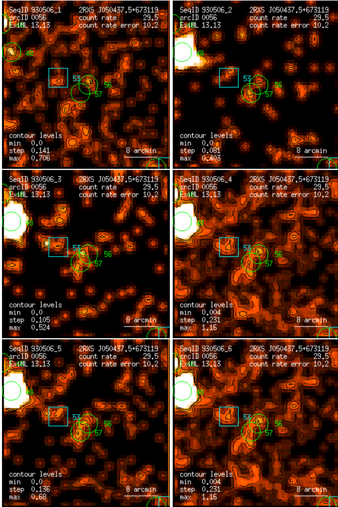
Figure 56: RASS 930506: detection 0056: band rate images, Gaussian filter: (1) PSPC channels 11 – 41, (2) 52 – 90, (3) 91 – 201, (4) 11 – 235, (5) 52 – 201, (6) 11 – 201. Broad band rates in counts/ks. Band rate contour levels in counts/ks/arcmin 2 .
