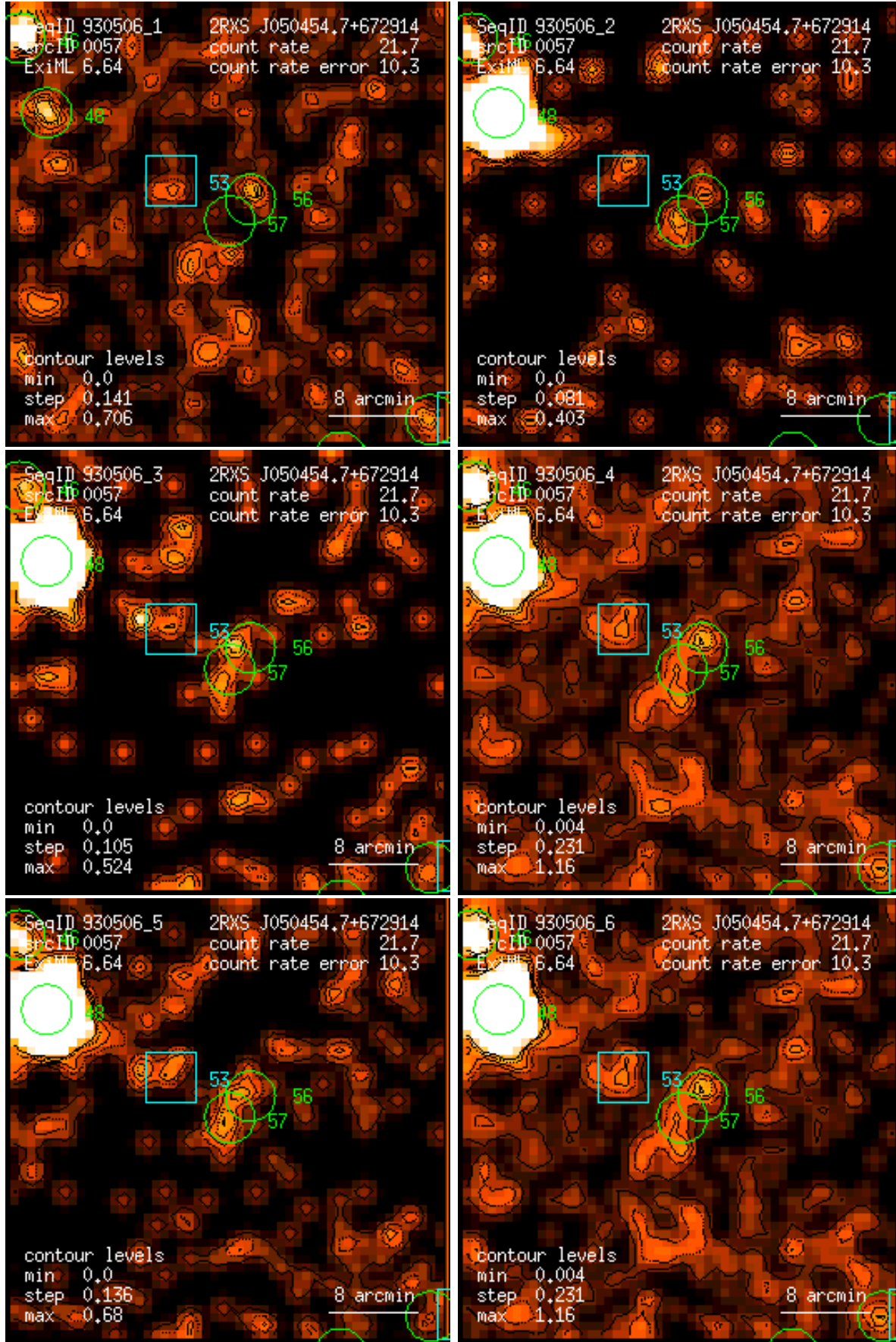
Figure 57: RASS 930506: detection 0057: band rate images, Gaussian filter: (1) PSPC channels 11 – 41, (2) 52 – 90, (3) 91 – 201, (4) 11 – 235, (5) 52 – 201, (6) 11 – 201. Broad band rates in counts/ks. Band rate contour levels in counts/ks/arcmin 2 .
