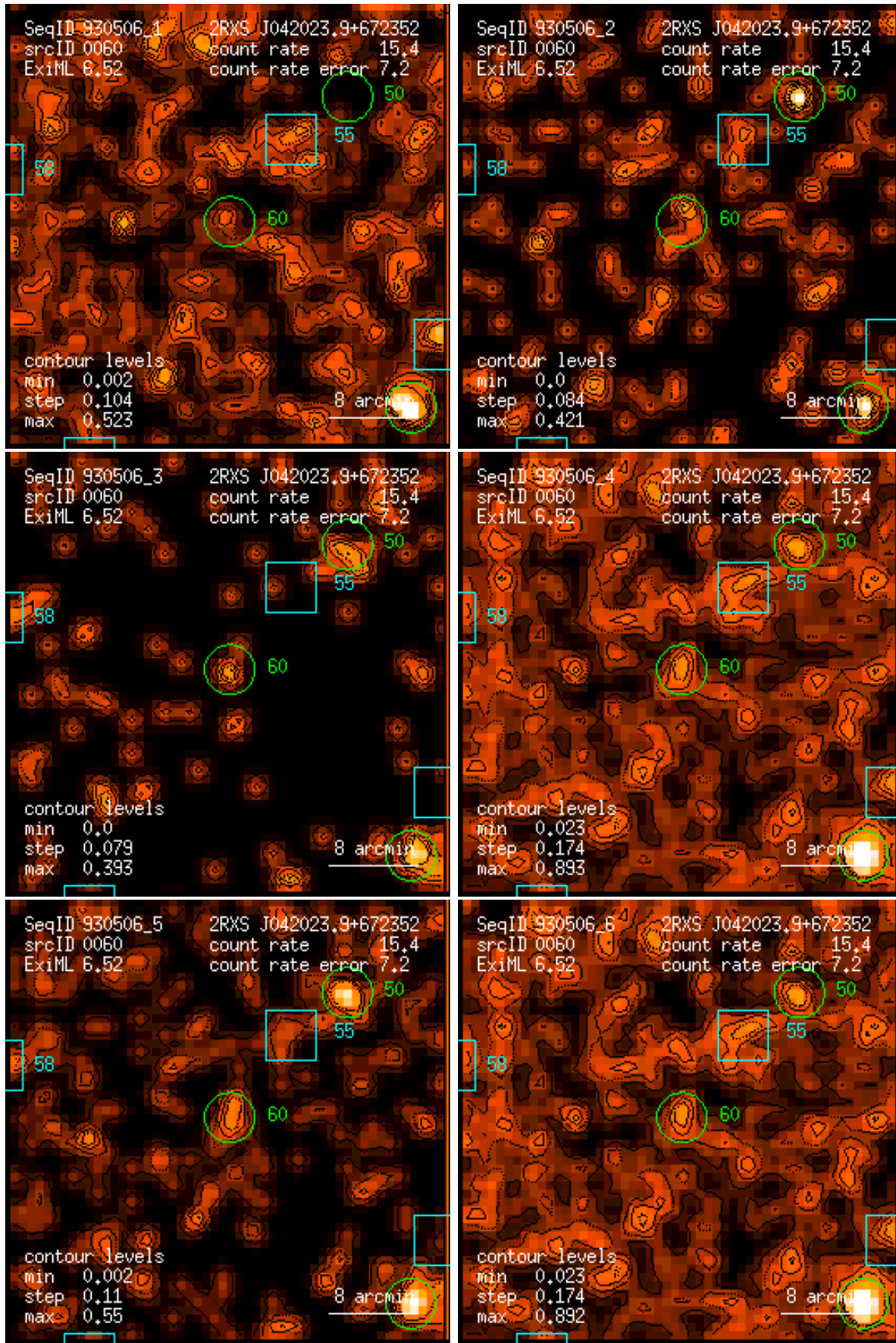
Figure 60: RASS 930506: detection 0060: band rate images, Gaussian filter: (1) PSPC channels 11 – 41, (2) 52 – 90, (3) 91 – 201, (4) 11 – 235, (5) 52 – 201, (6) 11 – 201. Broad band rates in counts/ks. Band rate contour levels in counts/ks/arcmin 2 .
