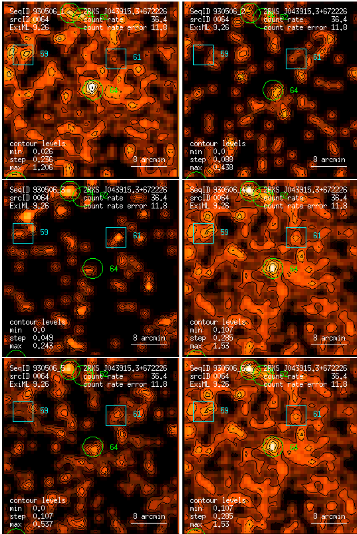
Figure 64: RASS 930506: detection 0064: band rate images, Gaussian filter: (1) PSPC channels 11 – 41, (2) 52 – 90, (3) 91 – 201, (4) 11 – 235, (5) 52 – 201, (6) 11 – 201. Broad band rates in counts/ks. Band rate contour levels in counts/ks/arcmin 2 .
