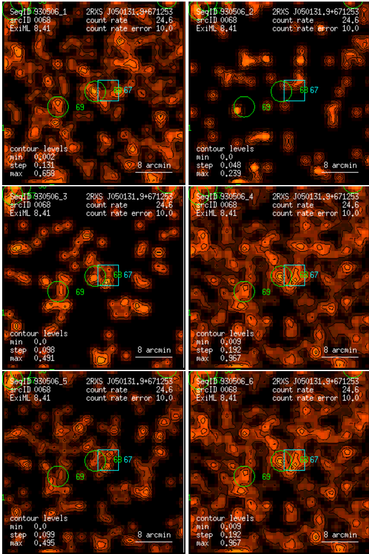
Figure 68: RASS 930506: detection 0068: band rate images, Gaussian filter: (1) PSPC channels 11 – 41, (2) 52 – 90, (3) 91 – 201, (4) 11 – 235, (5) 52 – 201, (6) 11 – 201. Broad band rates in counts/ks. Band rate contour levels in counts/ks/arcmin 2 .
